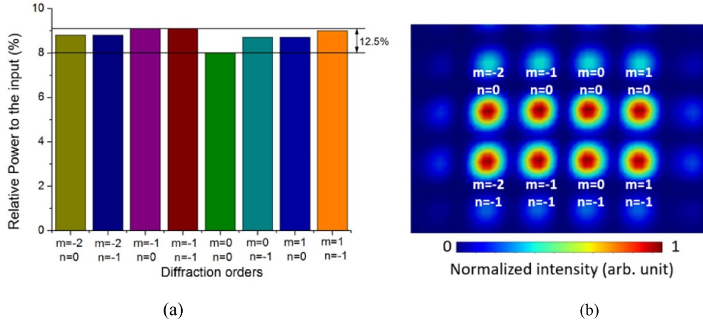
Figure 4. (a) Power distribution of the eight diffracted beams from the grating. The largest variation is 12.5% (between the maximum power and the minimum power). (b) Far field beam pattern of the grating, where m and n are the diffraction orders in two directions.
