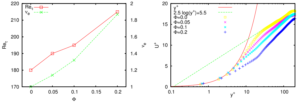
Figure 1. Left panel: friction Reynolds number Re_\tau and laminar effective viscosity (Eilers fit) \nu_e = \nu(1 + 1.25\phi/(1 - \phi/0.63)) vs volume fraction \phi . Right panel: Mean velocity profile normalized by the friction velocity U^+ = U/u_* vs wall normal distance rescaled in viscous units y^+ = y/(\nu/u_*) for different volume fractions.
