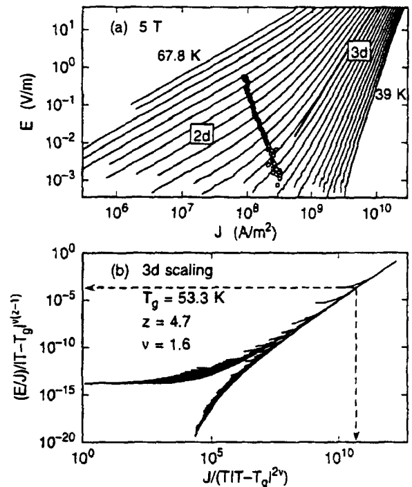
Figure 1. (a) Selected I - V isotherms for a 100 Å film. Curves are 1.2 K apart. Thick solid line denotes T_g . Open dots represent the crossover points where deviations from scaling occur. The data in the upper right corner (marked 3d) show the scaling behavior, whereas the data at lower left (2d) lead to deviations from scaling. (b) 3d scaling plot of the above data. Dashed lines illustrate the definition of points that characterize the crossover from 3d scaling to 2d deviations [open dots in (a)].
