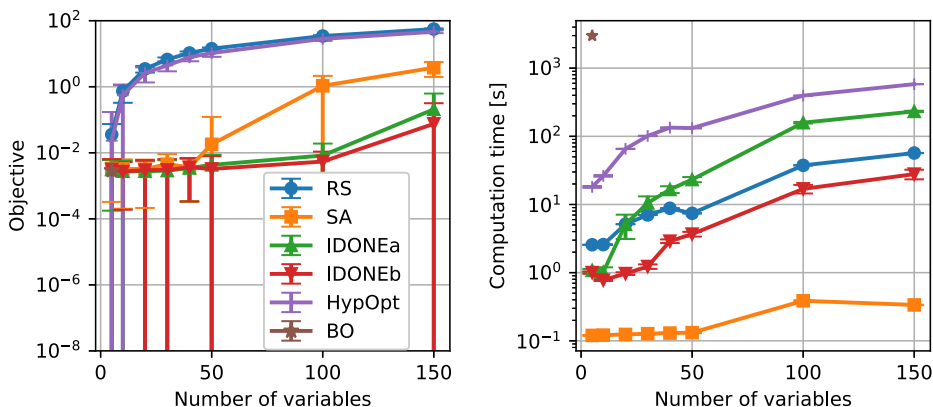
Fig. 5 Objective value ( left ) and computation time ( right ) of the convex binary optimization problem for the different algorithms after 1000 iterations, averaged over 100 runs, for problems with different numbers of variables d . Bayesian optimization (BO) was evaluated only for 1 run
