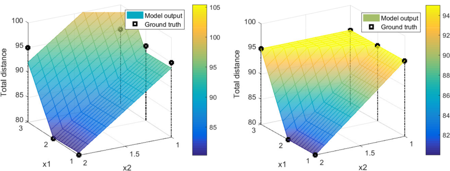
Fig. 2 Model output for the simple traveling salesman problem for the basic model (left) and the advanced model (right) . The starting city is city 1, x_1 determines which remaining city is visited next, x_2 determines which remaining city is visited third, then the only remaining city is visited, and then city 1 is visited again
