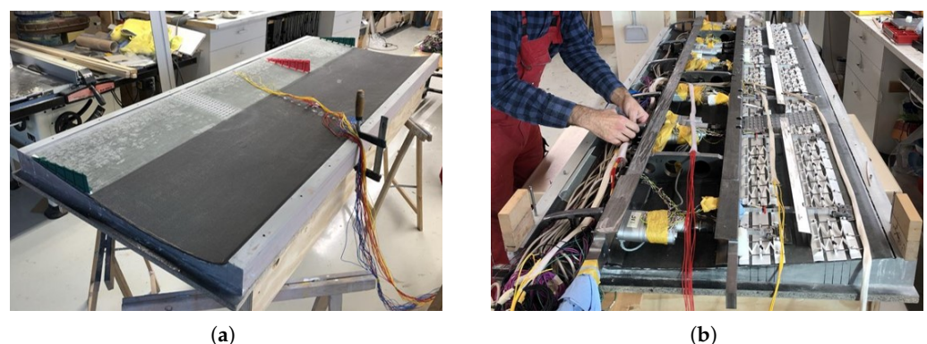
Figure 6. Prototype wing manufacturing. (a) Suction-side assembly. (b) Pressure-side assembly.
