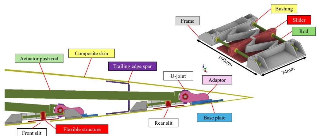
Figure 3. Trailing edge section view focusing on key components, including a focused view of the flexible structure segment.
