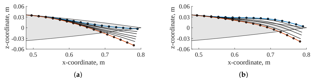
Figure 8. Reflexed morphing shapes. (a) Positively reflexed. (b) Negatively reflexed.
