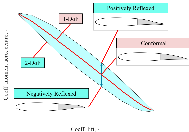
Figure 1. Schematic representation of the 2-DoF camber morphing functionality.
