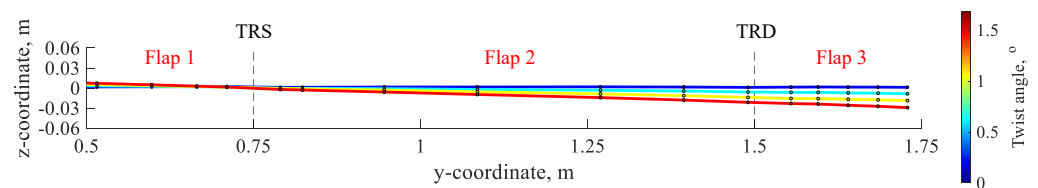
Figure 10. Twist morphing across the wing's trailing edge.
