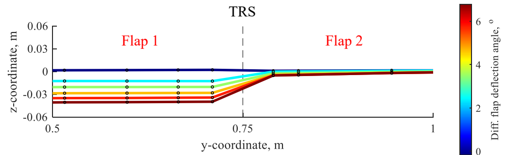
Figure 9. Asymmetric camber morphing between adjacent flaps.
