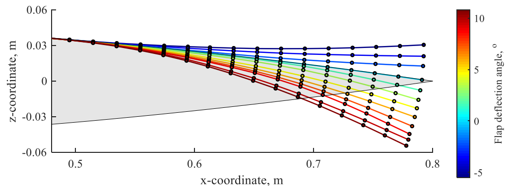
Figure 7. Conformal morphing shapes.
