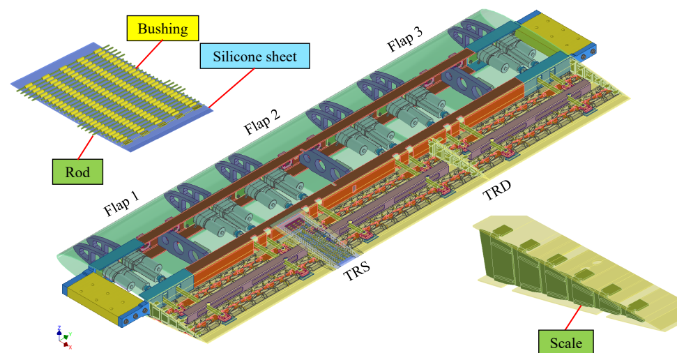
Figure 4. Prototype wing design focusing on TRS and TRD design.
