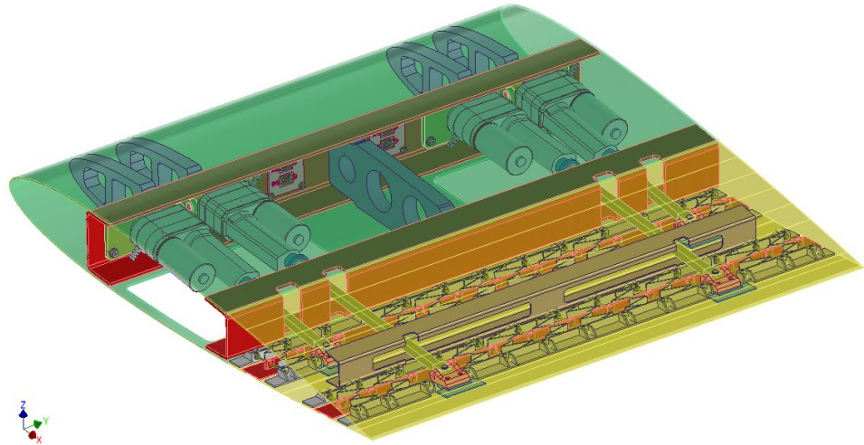
Figure 2. Morphing flap design.
