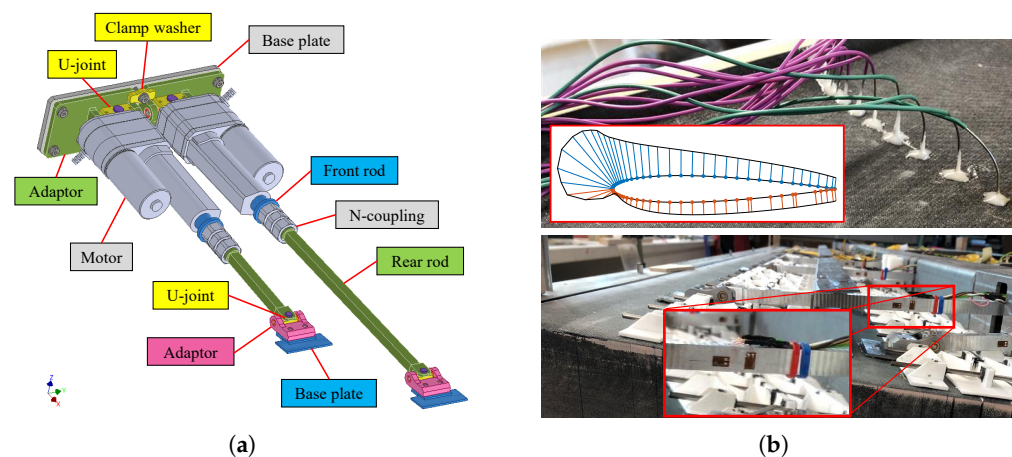
Figure 5. Onboard instrumentation. (a) Actuator assembly. (b) Pressure taps and load cells.
