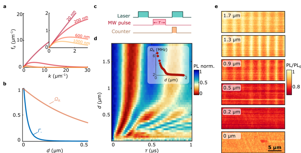
Figure 2. Tuning the NV-sample distance as a filter to selectively image a long-wavelength spin-wave mode. (a) The spin-wave stray field is proportional to a prefactor f_k (filter function) that depends on the NV-sample distance d (eq 1). The filter function peaks at k = 1/d , where k is the spin-wavenumber. The filter function is plotted for several values of d . (b) Calculation comparing the NV relaxation rate \Gamma_- caused by thermal spin waves to the NV Rabi oscillation rate caused by a coherently driven spin wave. Both rates are normalized to their value at d = 0 to highlight the different scaling with distance. The calculation of \Gamma_- assumes an equal population of all spin-wave modes at frequency f_- as expected for a Rayleigh-Jeans distribution. 21 The calculation of \Omega_R assumes only a single spin-wave mode with wavenumber k = 2 \mu\text{m}^{-1} (as imaged in e) is excited. (c) Pulse sequence used for the measurement in d: A 2.5 \mu\text{s} green laser pulse initializes the NV spin. A variable-duration microwave (MW) pulse excites spin waves. The final NV spin state is read out by measuring the NV photoluminescence during the first 600 ns of a second green laser pulse. (d) Spin-wave-driven NV spin dynamics vs tip-sample distance d . The dynamics are governed by the stray-field spectrum of the spin waves at the NV frequency. For d \gtrsim 100 \text{ nm} , the stray field of a coherent spin wave yields high-visibility Rabi oscillations with a long decay time. Below \sim 100 \text{ nm} , the Rabi decay time starts to vanish, attributed to the more rapidly increasing stray field generated by thermal spin waves (see b). Measurement taken at 31 \mu\text{m} from the stripline edge at B_0 = 32 \text{ mT} , f_- = 1.98 \text{ GHz} , and P_{\text{MW}} = 6.3 \text{ mW} . Inset: Fitted Rabi frequency vs d down to 100 \text{ nm} . (e) Spatial maps of the ESR contrast while driving spin waves at f_- = 1.89 \text{ GHz} and B_0 = 35 \text{ mT} ( k_1 = 1.7 \mu\text{m}^{-1} and k_2 = 22 \mu\text{m}^{-1} ) at P_{\text{MW}} = 1 \text{ mW} for varying d . The ESR contrast is obtained by normalizing the NV photoluminescence under microwave excitation (PL) to that without microwave excitation ( \text{PL}_0 ).
