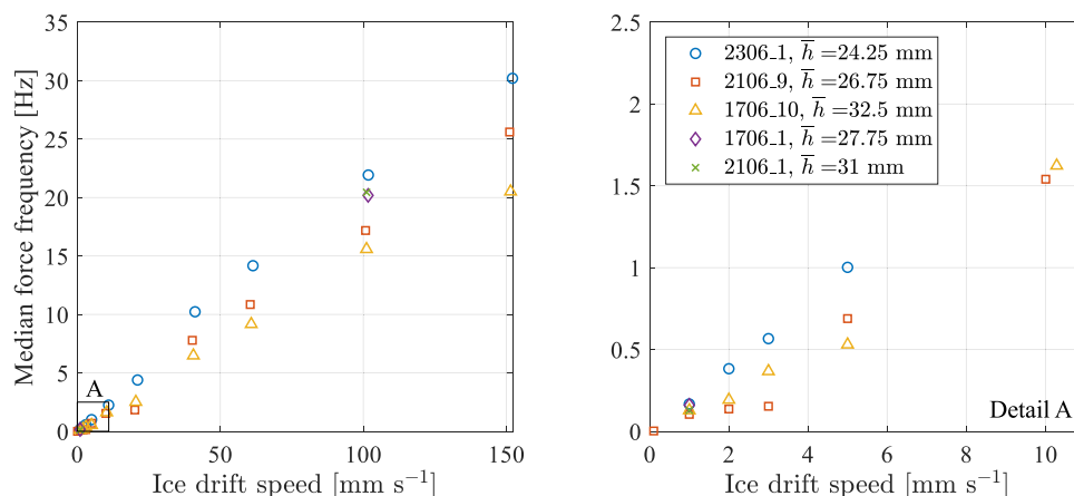
Fig. 3. Median ice force frequency as a function of drift speed.
