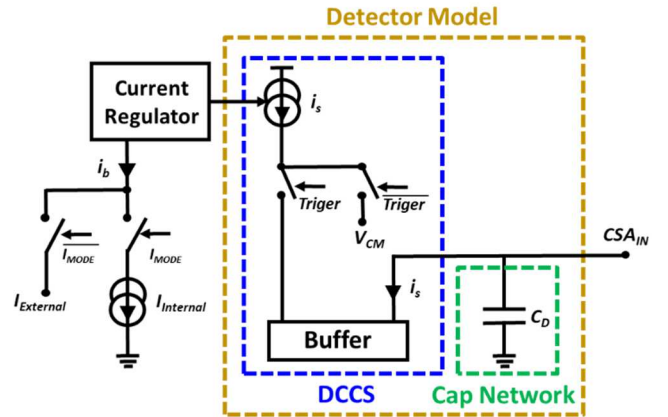
Fig. 4. Simplified schematic of the detector model.
