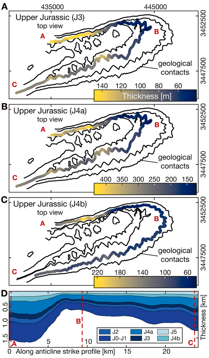
Fig. 8. Thickness model. (A/B/C) Model of thickness variations along contour lines of three Upper Jurassic sequences. (D) Modelled thickness variations of Jurassic rocks in a clockwise profile from the northwestern to the southwestern flank of the anticline.
