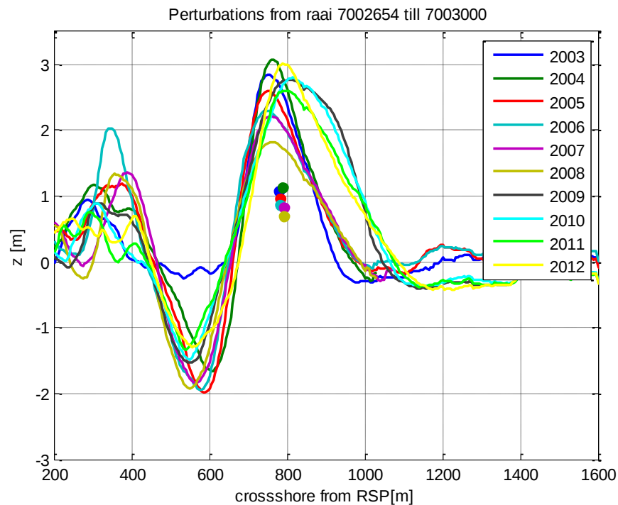
Figure 49: Perturbations of the blue cluster. The centroids remain on the same position (around 800m +RSP). This means that the shoreface nourishment remains in cross-shore direction on the same position.
