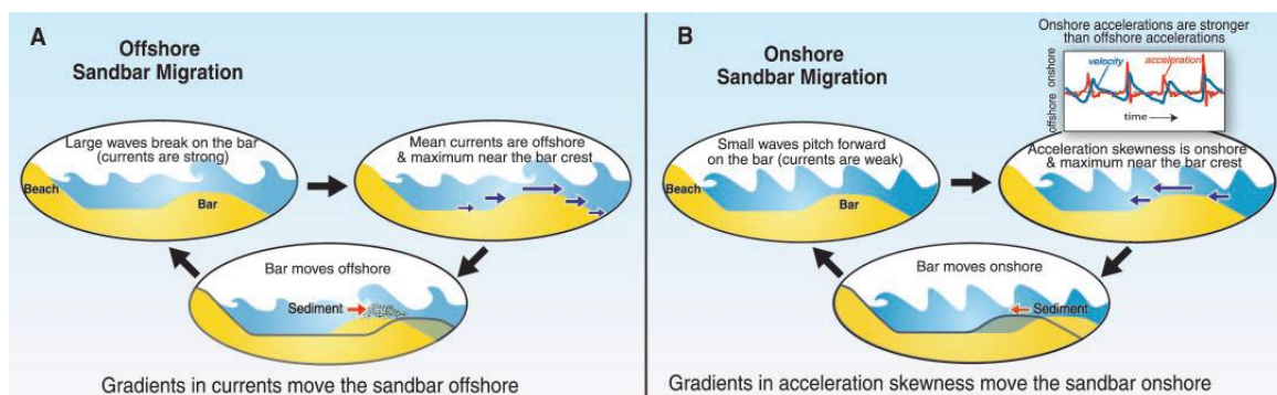
Figure 7: Driving processes that steer sandbar migration. In the left figure, the process for offshore migration is given and in the right figure, the process for onshore migration. (Hoefel, et al., 2003)
