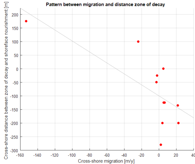
Figure 69: The correlation, -0.73 , between cross-shore migration shoreface nourishment and the distance between zone of decay and shoreface nourishment. A positive migration on the x-axis means a migration towards the coast and a positive distance at the y-axis means that the shoreface nourishment is executed onshore of the point of decay.
