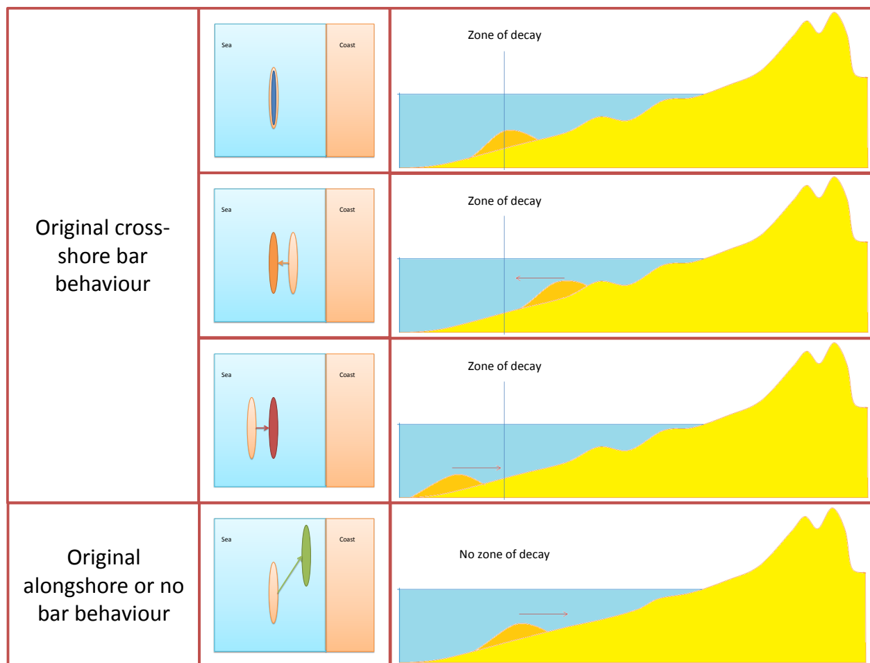
Figure 90: Overview of migration of shoreface nourishments (shown by the different clusters) in relation to the original bar behaviour.
