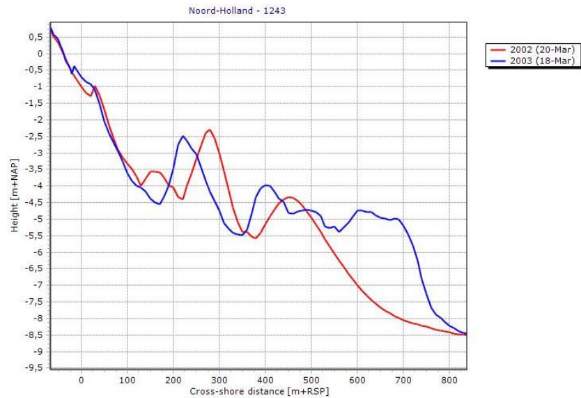
Figure 65: The profiles in 2002 (red) and 2003 (blue) for the shoreface nourishment at Callantsoog executed in 2001. This one is placed against the outer bar.
