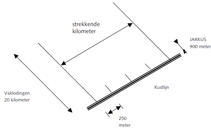
Figure 18: Visualisation of the differences between JARKUS and vaklodging. The JARKUS survey is performed each year with a distance of 250m and the vaklodgingen are performed every three year with a distance of 1000m. (Wiegmann, 2002)
