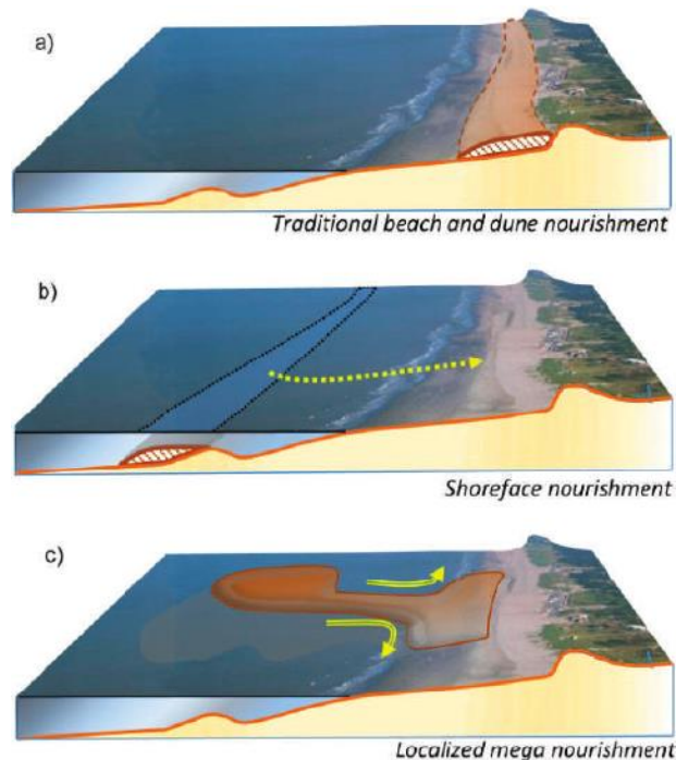
Figure 15: Types of nourishment. The first figure is a beach nourishment; the sand is placed at the beach. The second figure is a shoreface nourishment; the sand is placed between -8 m and -5 m NAP. The third figure is a mega nourishment; the sand motor is a good example of this type. (Stive, et al., 2013)
