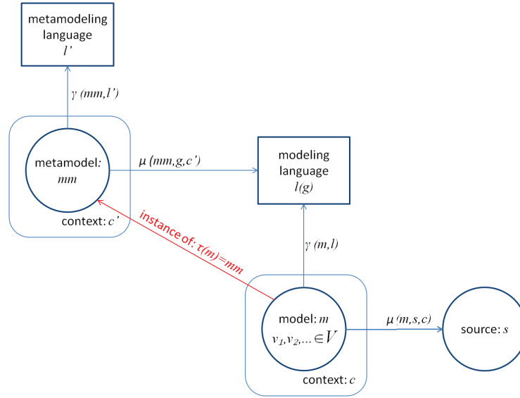
Fig. 2. Metamodeling.
