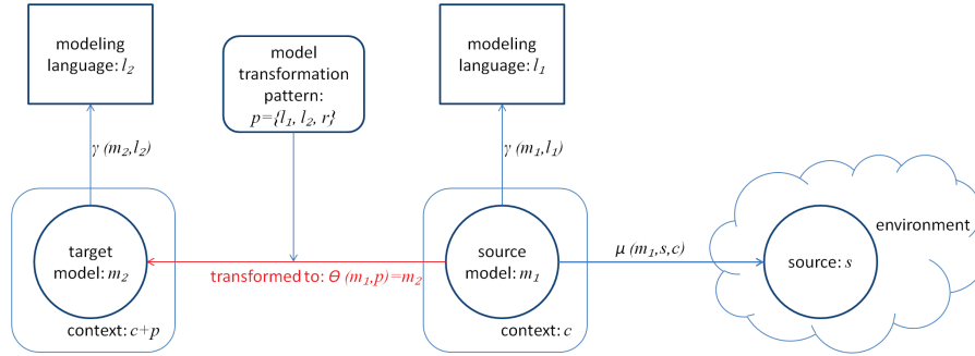
Fig. 3. The relationships in a model-to-model transformation.
