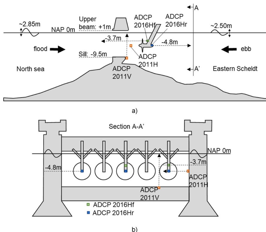
Fig. 3. a) A cross section through the middle turbine in Gate 8 of the Rooppot Section of the Eastern Scheldt barrier. The location and orientation of the ADCP's on the turbines and the ADCP's applied in 2011 on the barrier are indicated (2011H: horizontal out of plane and 2011V: vertical) and the ADCP's on the turbines in 2016 are indicated by ADCP2016Hf: front ADCP and ADCP2016Hr: rear ADCP. The length of the arrows show the measurement range of the ADCP's. All levels refer to NAP. Fig. 3b: Cross section over the width of Rooppot Gate 8.
