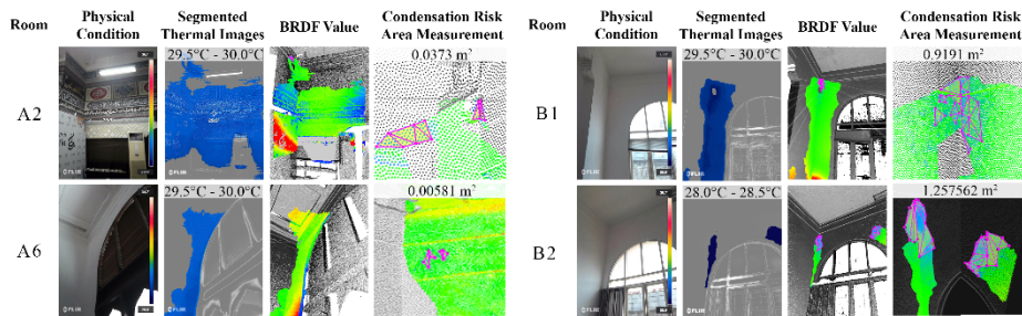
Figure 5. Condensation risk area based on surface temperature and BRDF
