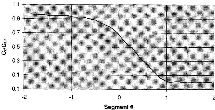
Fig. 8-9 Measured capacitance ratio versus interface level for conductive liquids
