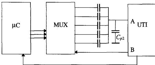
Fig. 6-18 Block diagram of the system using the UTI from Smartec
