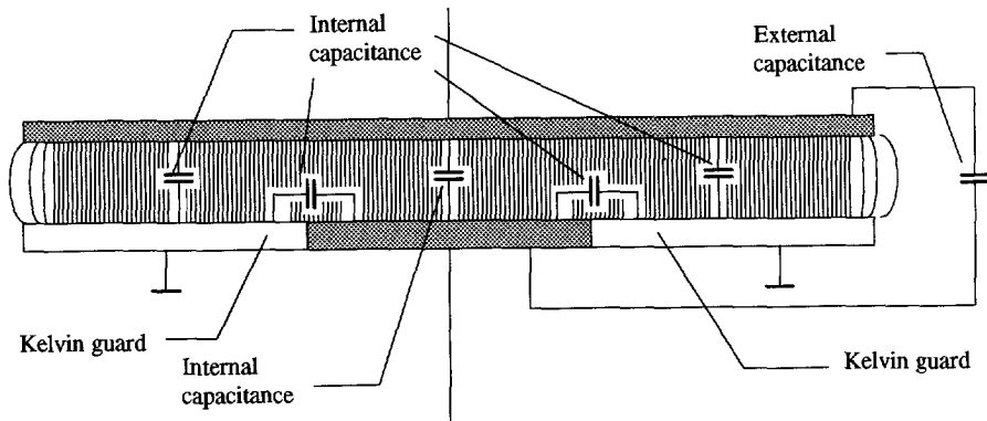
Fig. 5-14 Simple parallel plate capacitor with Kelvin guard electrode
