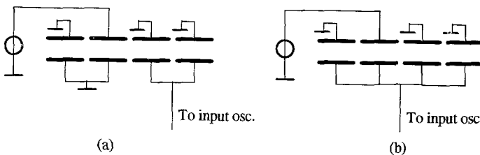
Fig. 5-22 Right-half cross-section of the electrode structure for measuring (a) cross-capacitance and (b) trans-capacitance
