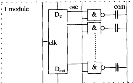
Fig. 8-7 Multiplexer circuit for capacitances
