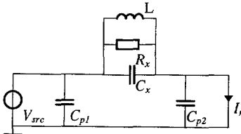
Fig. 6-9 Resonance method
