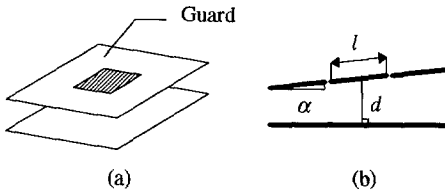
Fig. 5-8 Parallel plate capacitor (a) perspective (b) cross-section
