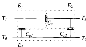
Fig. 5-2 Static electrical model for a multi-electrode capacitor
