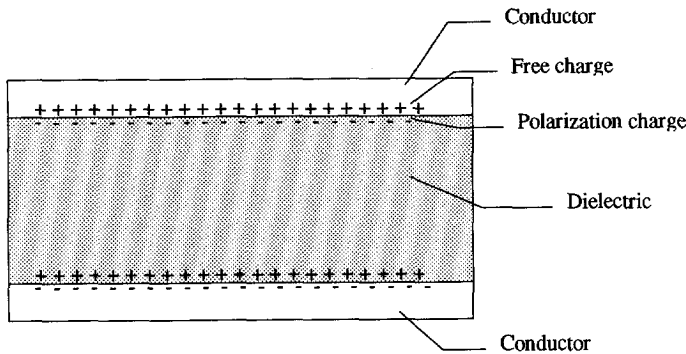
Fig. 5-1 Dielectric placed between two conductors kept at a constant potential difference
