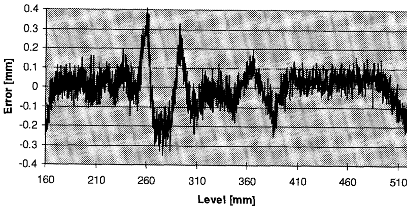
Fig. 8-12 The total error for Euro Super over a measurement range of 300 mm
