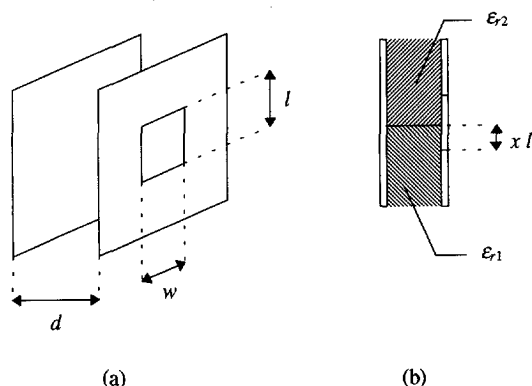
Fig. 8-2 Biplanar capacitor filled with two substances (a) perspective (b) cross-section
