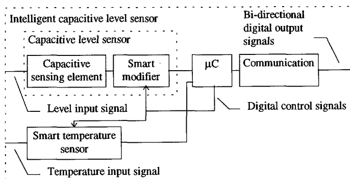
Fig. 8-1 Data flow diagram for the intelligent capacitive level sensor system
