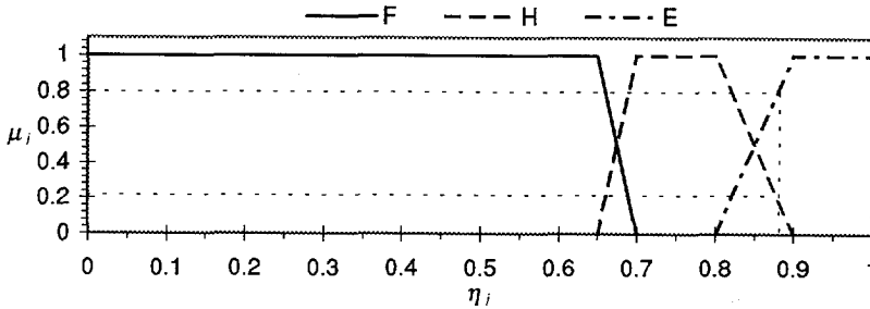
Fig. 9-6 Memberships function of the groups F, H and E
