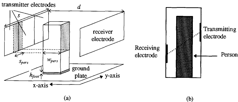
Fig. 9-1 Simplified model of the electrode structure, (a) perspective of the position sensor (b) cross-section of the entrance detector
