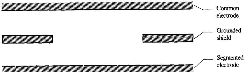
Fig. 5-10 Cross-section of multi-electrode biplanar structure with grounded shield
