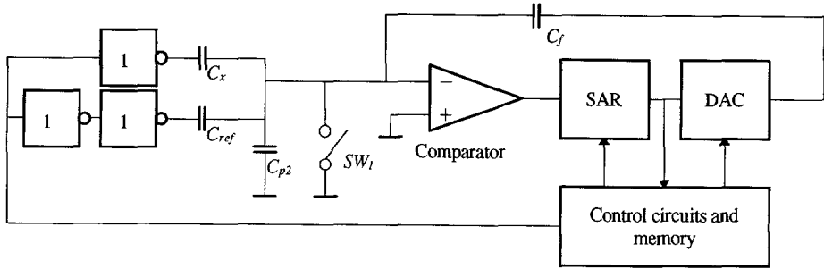
Fig. 6-11 Charge amplifier presented by Kung et. al.
