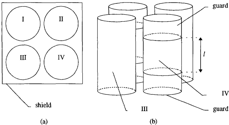
Fig. 5-6 Thompson and Lampard standard capacitors (a) top view (b) perspective
