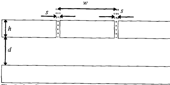
Fig. 5-19 Cross-section of a parallel plate capacitor with guard electrodes and finite gap widths
