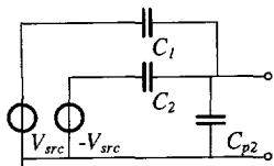
Fig. 6-8 Bridge imbalance measured with a voltage meter
