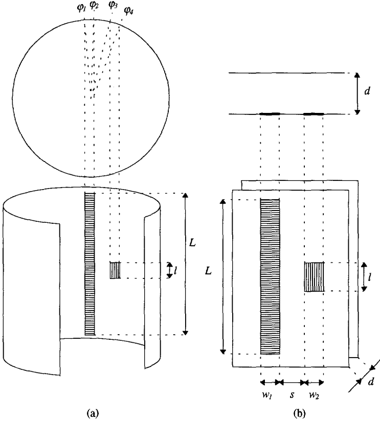
Fig. 5-11 Cylindrical (a) and uniplanar (b) square-strip electrode structures
