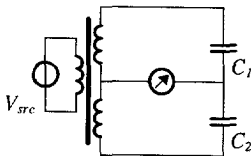
Fig. 6-7 Bridge circuit with 3-winding transformer
