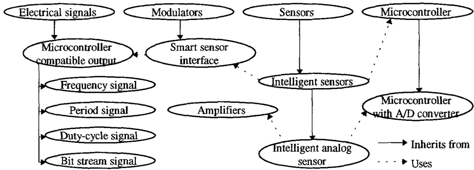
Fig. 4-5 Class diagram for intelligent sensors
