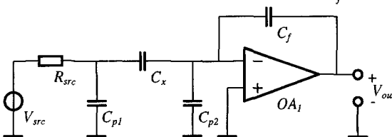
Fig. 6-2 Circuit to reduce the influence of C_{p2} and C_{p3}
