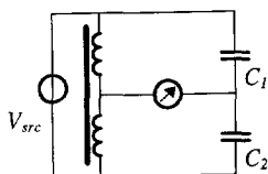
Fig. 6-6 Bridge circuit with 2-winding transformer
