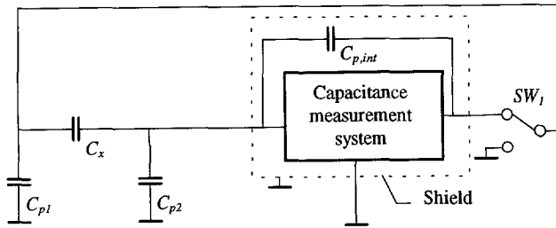
Fig. 6-4 Using an output multiplexer to keep in total input capacitance constant
