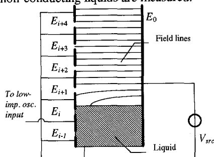
Fig. 8-4 Conductive liquid connected to ground
