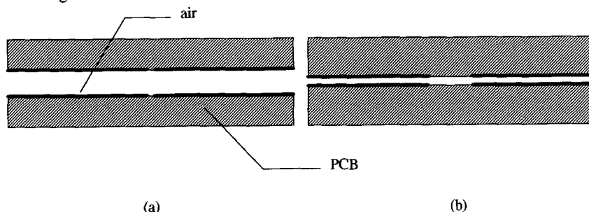
Fig. 5-18 Cross-capacitors with thin electrodes on printed circuit board, (a) with thin gaps and (b) with wide gaps
