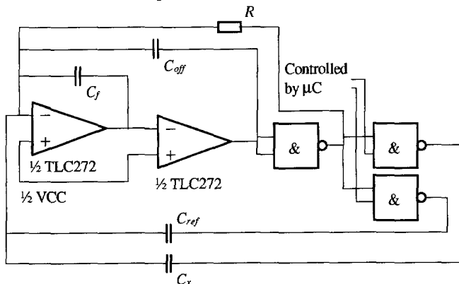
Fig. 8-6 The modified Martin oscillator
