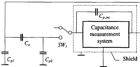
Fig. 6-1 Identification of parasitic capacitances
