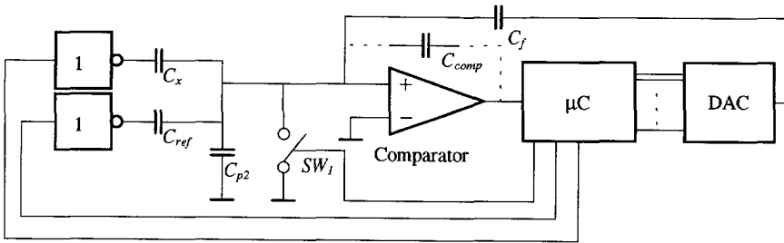
Fig. 6-19 Smart charge redistribution
