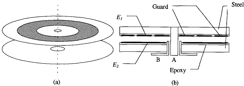
Fig. 7-4 The proposed capacitive sensing element (a) perspective (b) cross section
