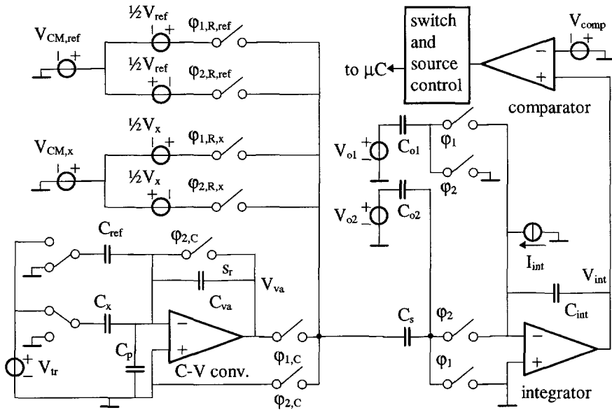
Fig. 6-17 Multiple-sensor modulator in capacitance measurement mode (reprinted from [8])
