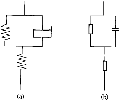
Fig. 7-6 Mechanical (a) and equivalent electrical model (b) for time-dependent anelastic deformation
