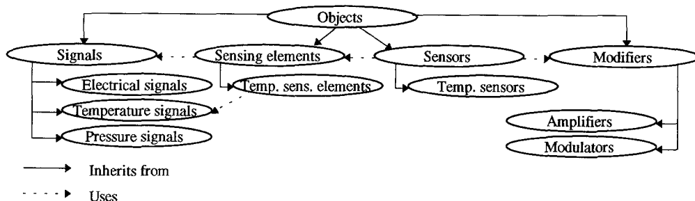
Fig. 4-4 Class diagram for signals, modifiers, sensing elements and sensors
