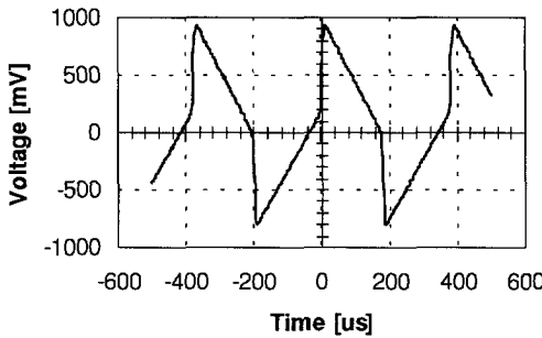
Fig. 6-14 Measured output signal of the integrator
