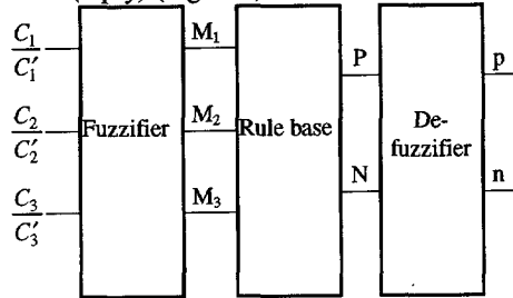
Fig. 9-5 Fuzzy logic data flow
