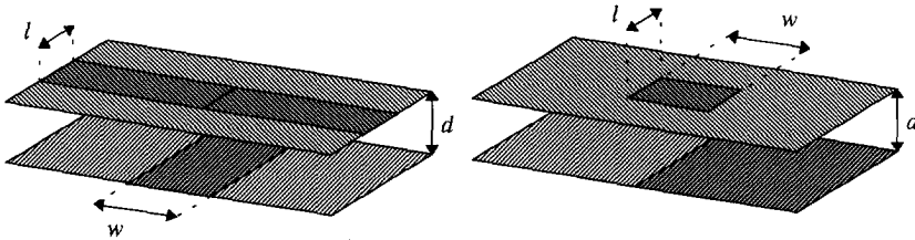
Fig. 5-9 Differential biplanar electrode structures
