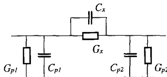
Fig. 5-13 Electrical model in the case of slightly conducting fluids in direct contact with the electrodes
