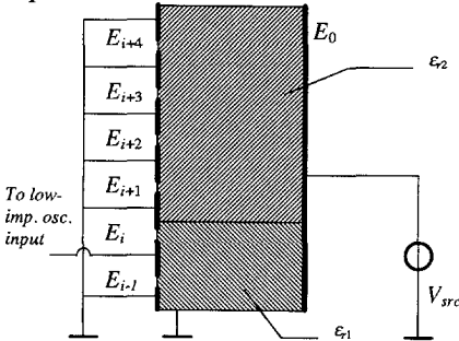
Fig. 8-3 Multi-electrode structure where C_i is measured
