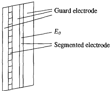
Fig. 8-5 Novel planar electrode structure
