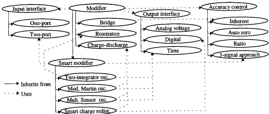
Fig. 6-20 Class diagram for smart modifiers
