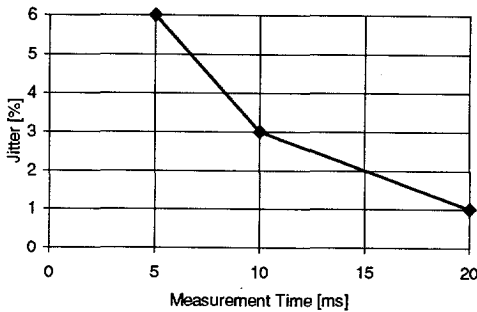
Fig. 9-8 Jitter of the measurement system versus measurement time
