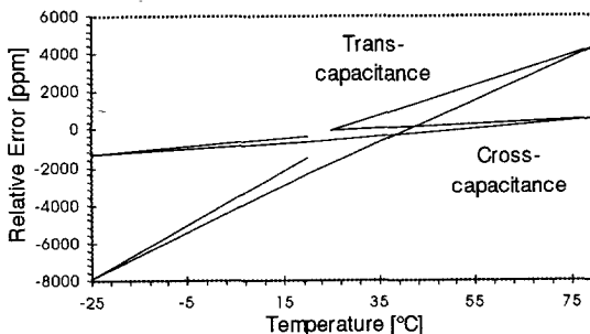
Fig. 7-9 Temperature effects on the circular cross-capacitor and the circular trans-capacitor
