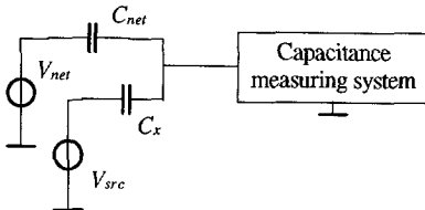
Fig. 6-5 Electrical model for LF interference
