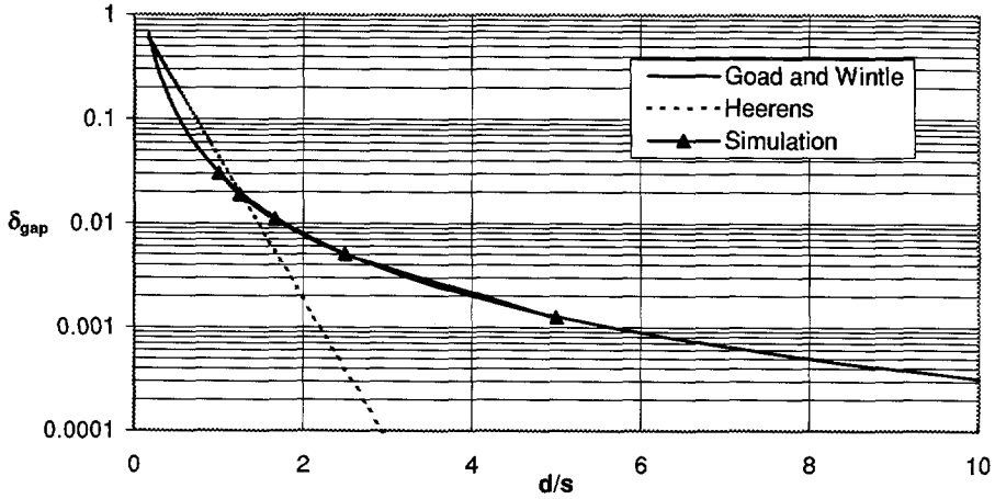
Fig. 5-20 Gap error according to Heerens, Goad and Wintle and simulations
