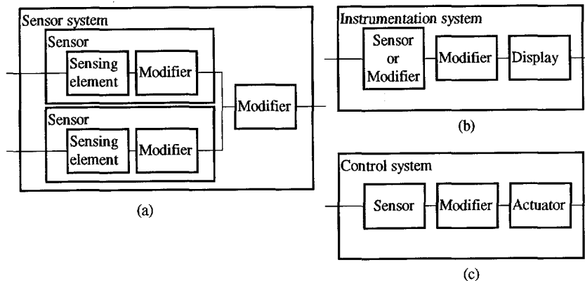
Fig. 4-3 (a) Sensor system (b) Instrumentation system (c) Control system
