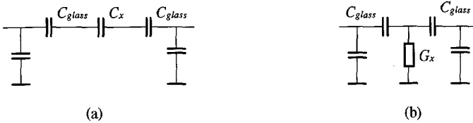
Fig. 5-12 Electrical model with series capacitances in the case of (a) non-conducting and (b) conducting liquids
