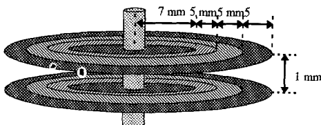
Fig. 5-21 Experimental circular cross-capacitor
