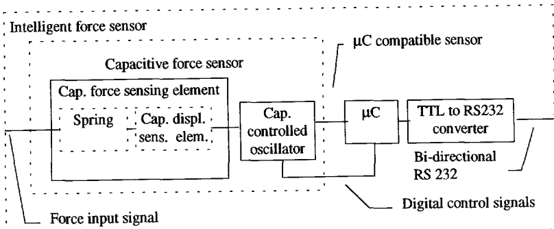
Fig. 7-3 Data flow diagram for an intelligent force sensor
