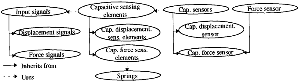
Fig. 7-1 Class diagram for capacitive displacement and force sensors and sensing elements
