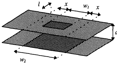
Fig. 5-15 Biplanar square-strip geometry
