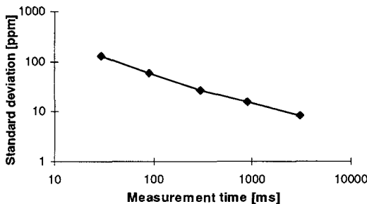
Fig. 6-16 Measured jitter as a function of the measurement time
