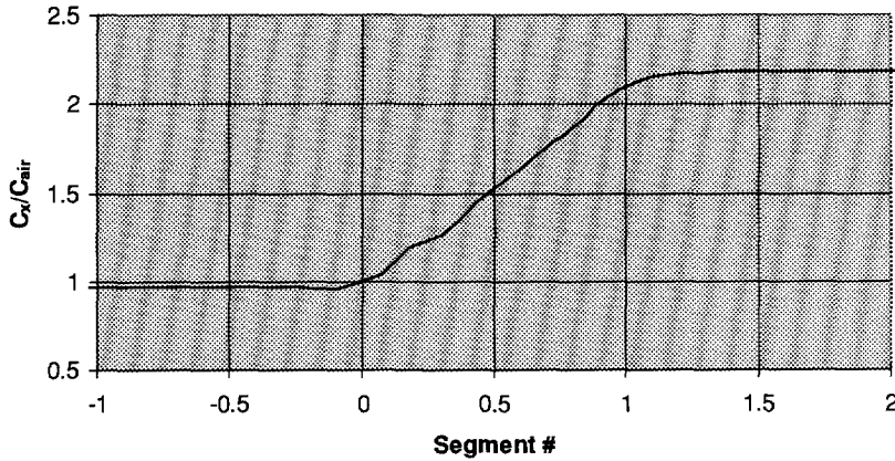
Fig. 8-10 Measured capacitance ratio versus interface level for non-conductive liquids
