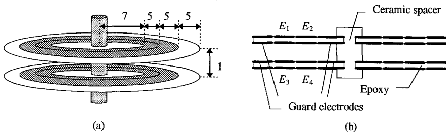
Fig. 7-5 Proposed circular cross-capacitor (a) perspective (b) cross-section
