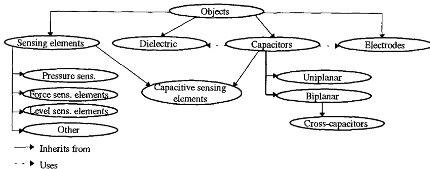
Fig. 5-24 Class diagram for capacitive sensing elements
