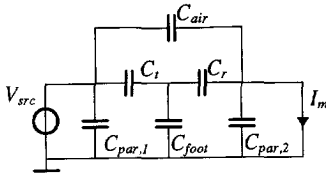
Fig. 9-2 Simple electric model of the structure
