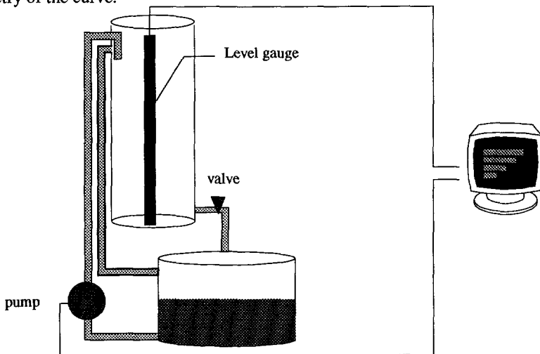
Fig. 8-11 Experimental setup
