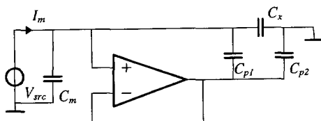
Fig. 6-3 1-port measurement with active guard
