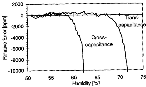
Fig. 5-23 Increasing humidity with 0.2%/min. at 80°C
