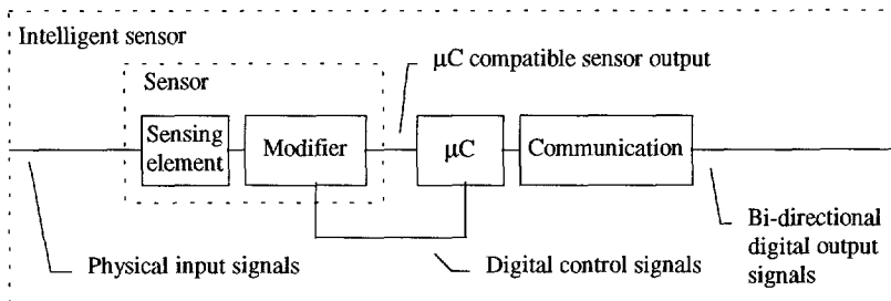
Fig. 4-6 Generic data flow diagram for an intelligent sensor
