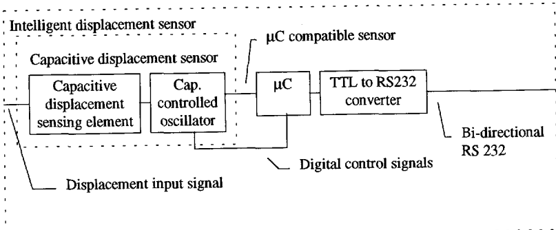
Fig. 7-2 Data flow diagram for an intelligent displacement sensor
