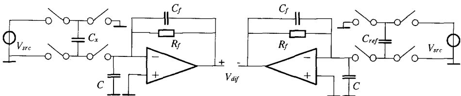
Fig. 6-10 Charge/discharge method
