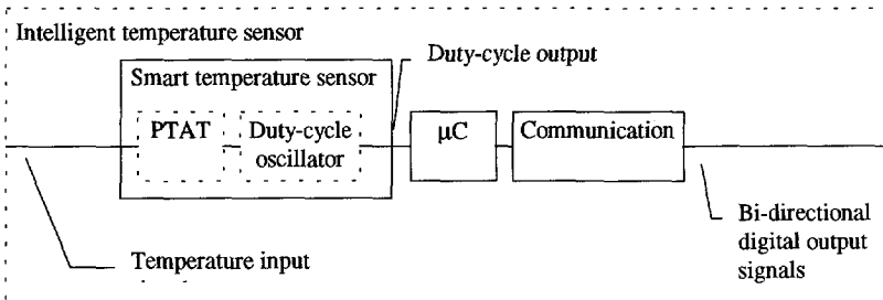
Fig. 4-7 Data flow diagram for an intelligent temperature sensor
