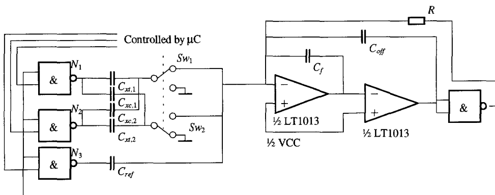
Fig. 6-15 Martin oscillator with double-sided multiplexing
