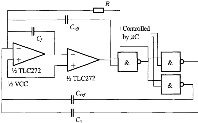
Fig. 6-13 Modified Martin oscillator
