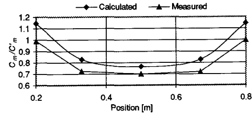
Fig. 9-4 Relative capacitance as function of the position on the x-axis of the person
