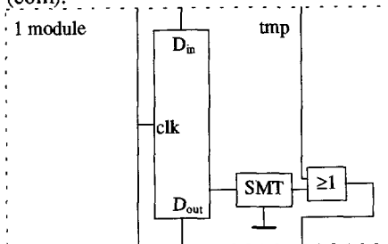
Fig. 8-8 Multiplexer circuits for Smartec temperature sensors
