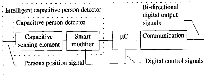
Fig. 9-3 Data flow diagram for the intelligent capacitive person detector
