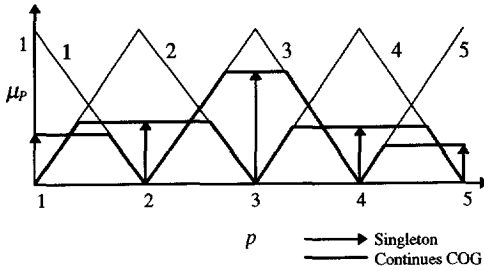
Fig. 9-7 Defuzzification using singletons
