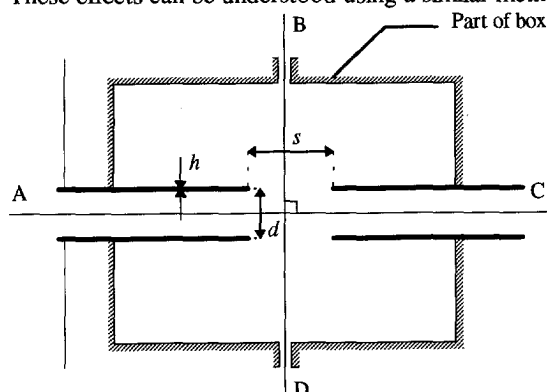
Fig. 5-17 Cross-section of a cross-capacitor with infinitely thin electrodes
