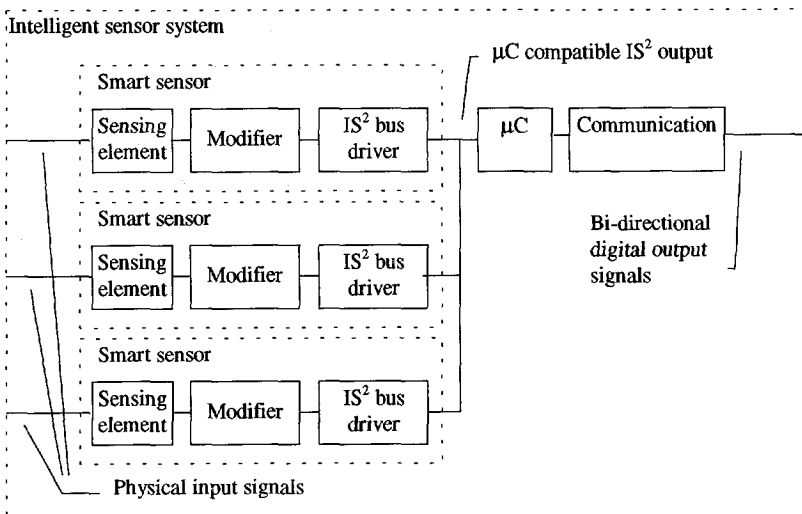
Fig. 4-8 Generic data flow diagram for an intelligent sensor system with IS^2 bus
