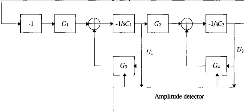
Fig. 6-12 Two-integrator oscillator
