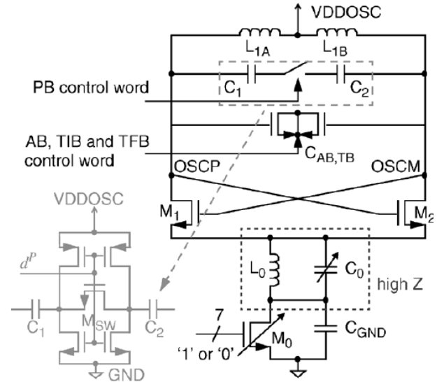
Fig. 1. DCO with capacitive tuning [4].
