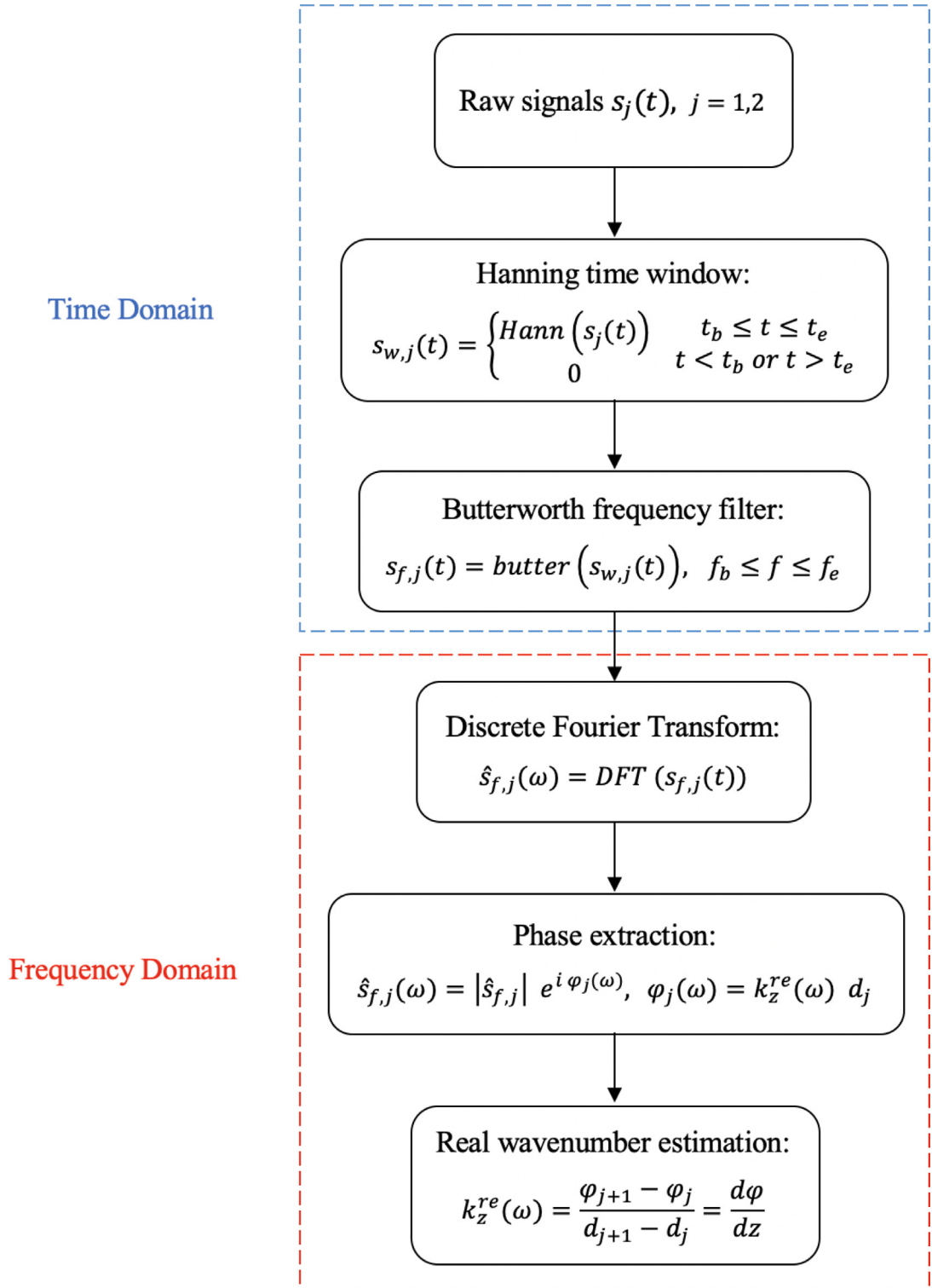
Fig. 2. The flowchart of the process used to estimate the real wavenumber k_z^{re} from the raw signals. The subscripts “b” and “e” denote the upper and lower limits in time windowing and frequency filtering. \phi_j is the extracted phase of a signal, d_j is the distance between the excitation point and the point of signal reception, d\phi and dz are the phase difference and distance between two receiving signals respectively, and i = \sqrt{-1} .
