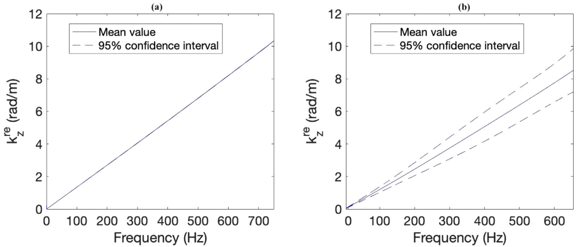
Fig. 6. The real part of the axial wavenumber k_z^{\text{re}} as a function of frequency for Set-up A (a) and Set-up B (b). k_z here represents the wavenumber of the axisymmetric fluid-borne wave. The results were obtained by processing the raw signals according to the procedure described in Fig. 2.
