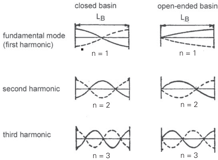
Figure 5.26 Basin oscillation
