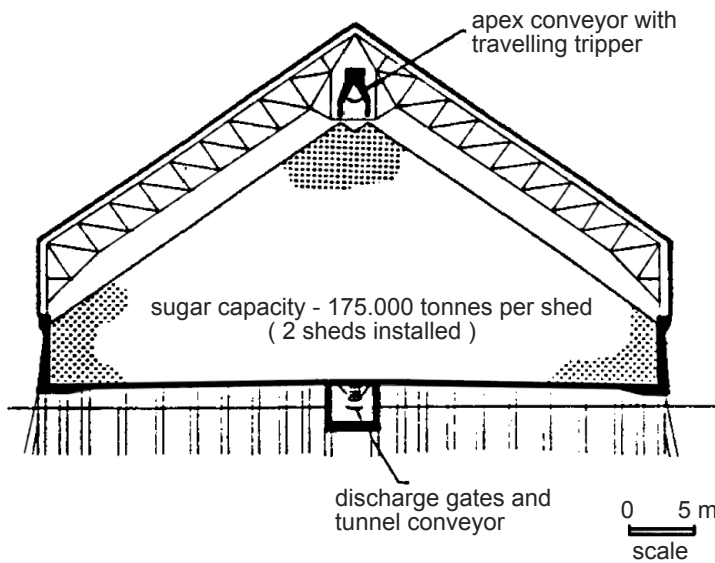
Figure 11.17 Storage shed
