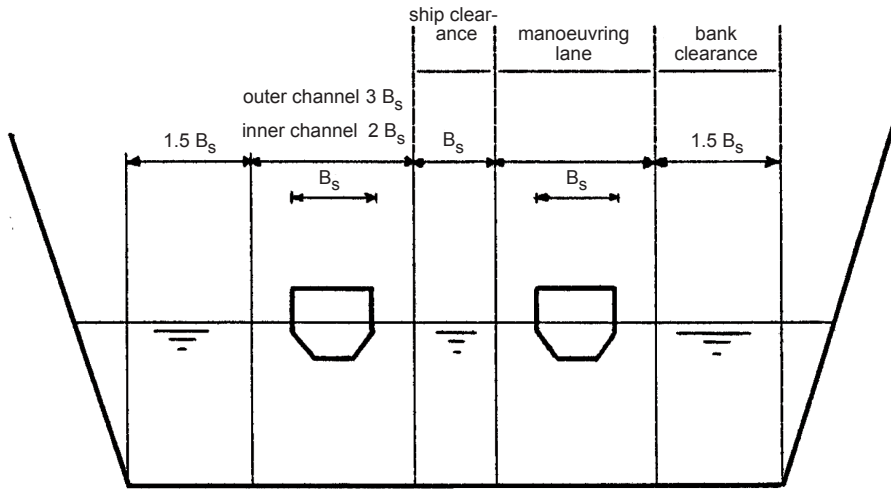
Figure 12.5 Channel width
