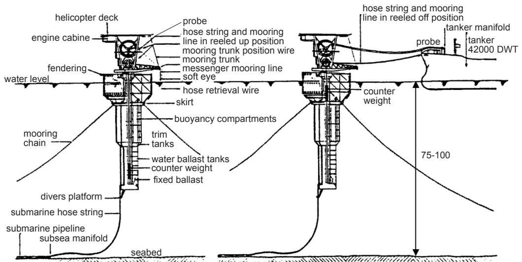
Figure 10.16 Deepwater SBM
