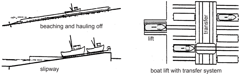
Figure 12.12 Dry-docking arrangements
