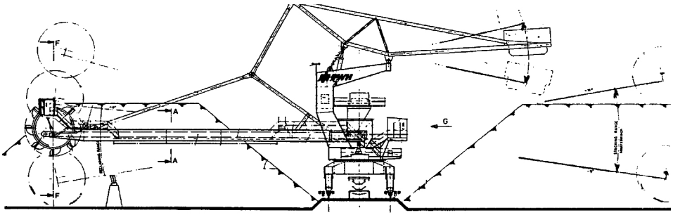
Figure 11.19 Stacker-reclaimer
