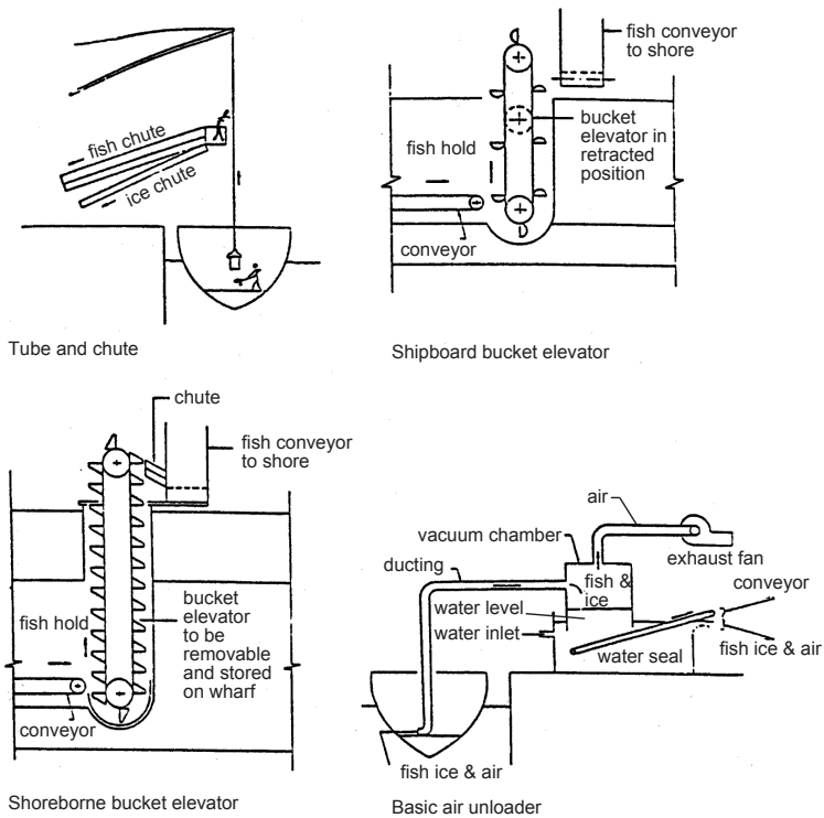
Figure 12.18 Unloading equipment
