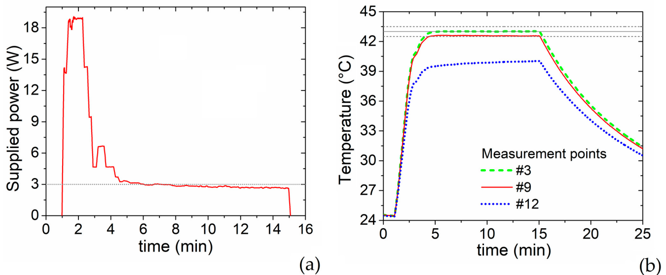
Figure 6. (a) Time evolution of the power effectively supplied to the RF applicator to perform steady-state measurements at 43 °C. (b) Consequent heating-cooling transients, measured in points #3, #9 and #12. The target temperature of 43 °C is indicated with a solid dark grey line, while the dashed lines indicate a \pm 0.5 °C difference from the target temperature.
