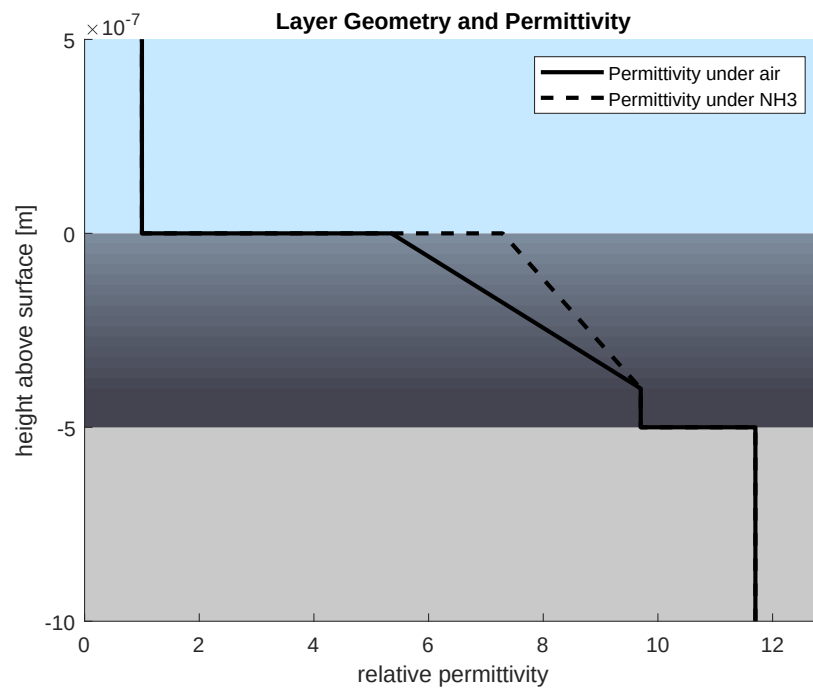
Figure 5.4: Permittivity distribution with depth with and without the presence of \text{NH}_3 gas following from the porosity model.
