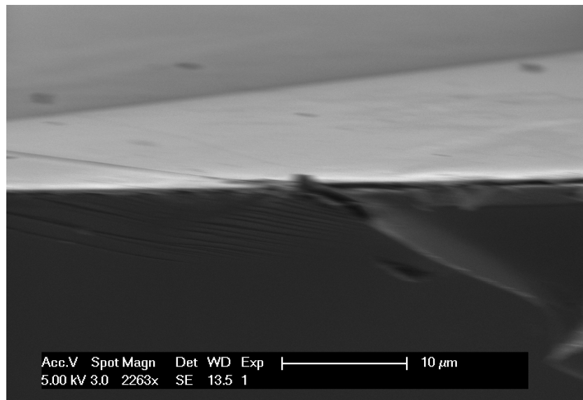
(c) Close up of the crack from a side view
