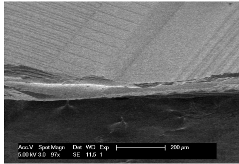
(a) Crack location as viewed under the SEM
