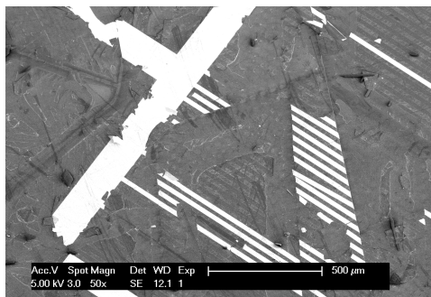
(a) SEM Image displaying the extensive damage to the electrodes caused by the etching process
