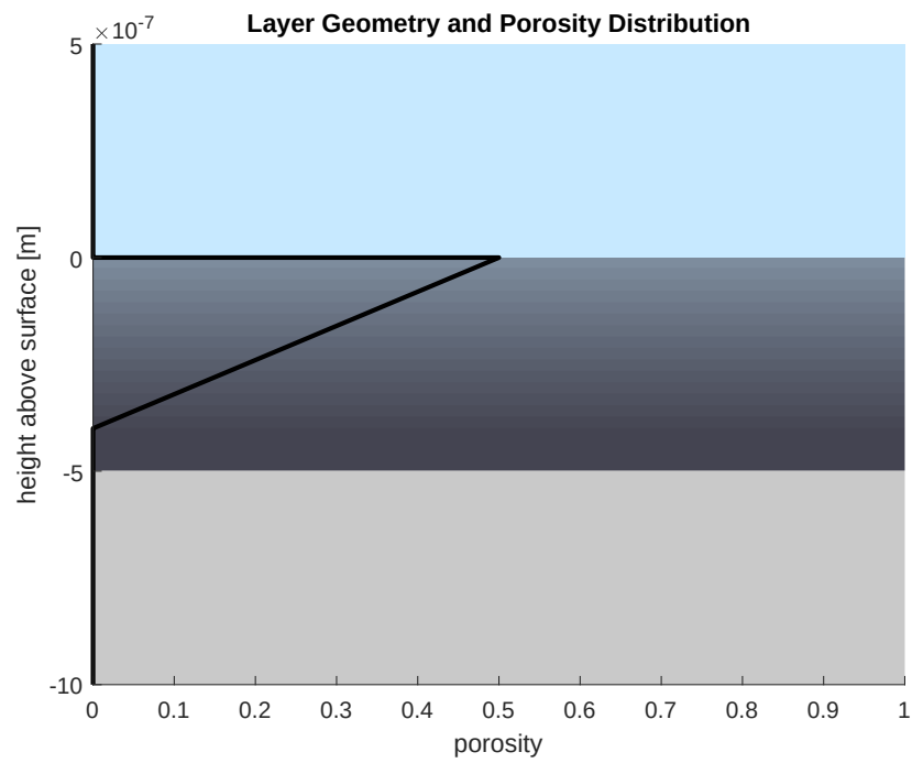
Figure 5.3: Distribution of porosity with depth within the SiC layer following from the porosity model.
