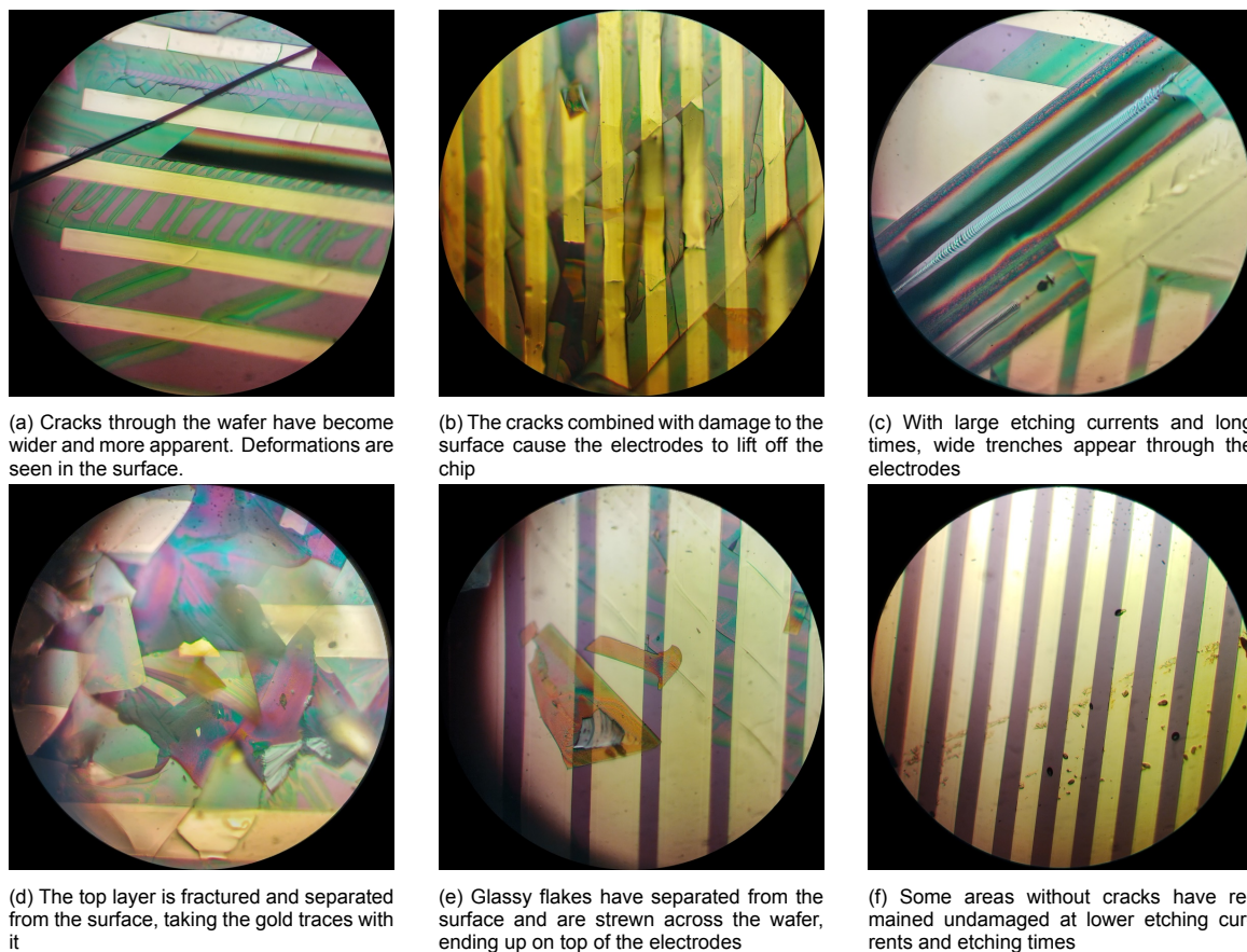
Figure 8.9: Microscope photographs of traces on various areas of the etched dies
