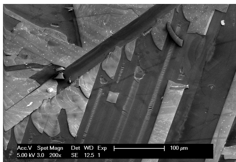
(e) Image showing the parallel lines near the die edge at an angle.
