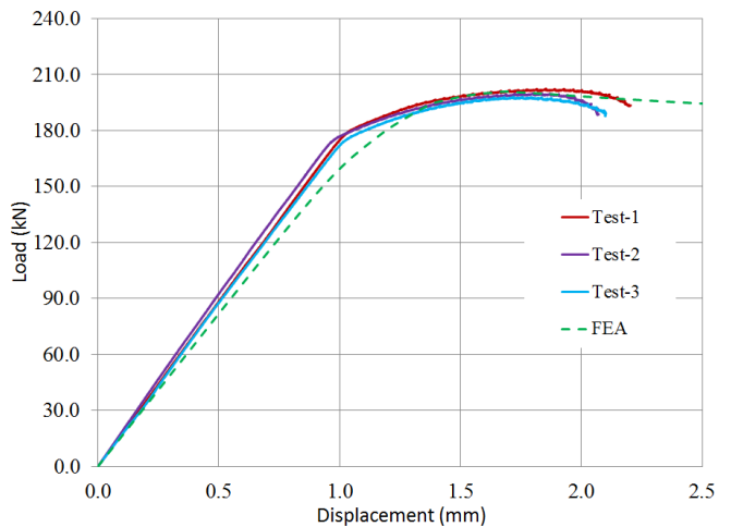
Fig. 14 Load-displacement curves obtained from the FEA and test results for 4 mm thick specimens with 120° cold-formed angle
