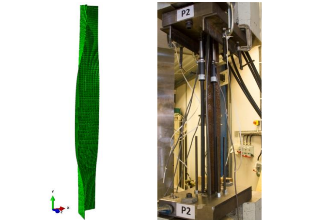
Fig. 15 Deformation of the 4 mm thick specimen with 100° cold-formed angle (FEA and experimental results)
