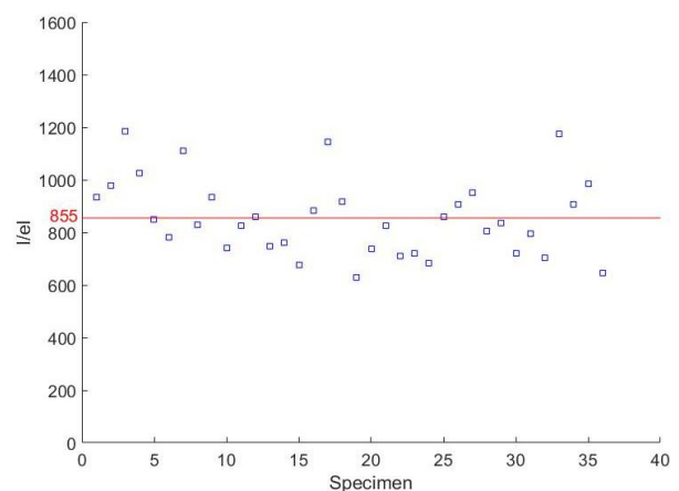
Fig. 12 Ratio between maximum initial geometric imperfection at the middle and length of each specimen
