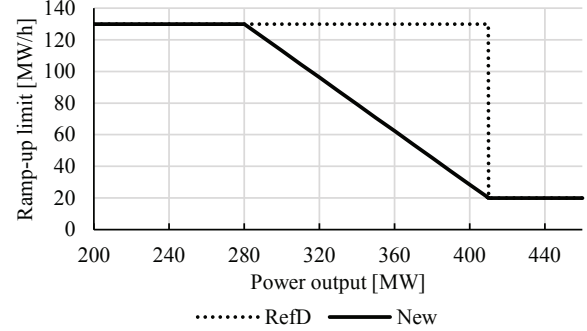
Fig. 3: Ramp-up limit vs. Power output
