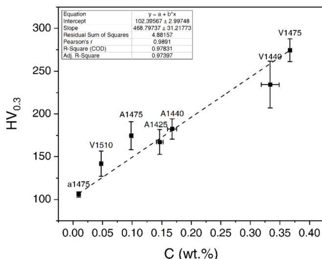
Fig. 23. Correlation among microhardness and carbon content.
