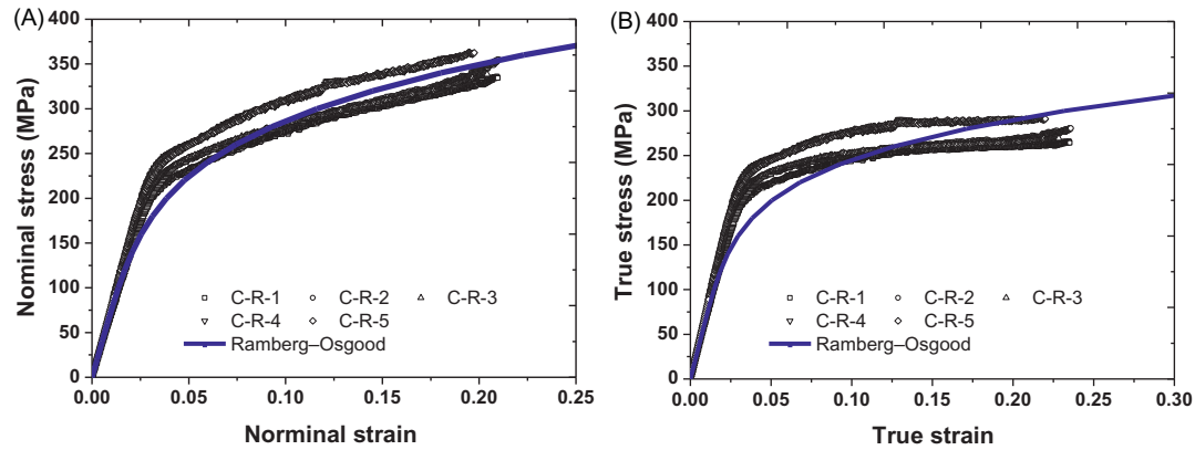
Figure 23.9 Stress—strain relationship of confined resin specimens: (a) Nominal stress versus nominal strain and (b) True stress versus true strain.
