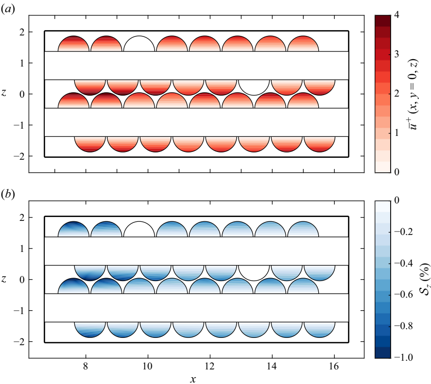
Figure 6. Spatial variations of (a) the streamwise wall velocity at Re_{\theta,1} = 1980 ( Re_{\tau,avg} = 880 ) and (b) the direct-slip term S_z(x, z) , defined in (4.1) using l(x) = 4.54\theta_0(x) , relative to C_{f,0}/2 .
