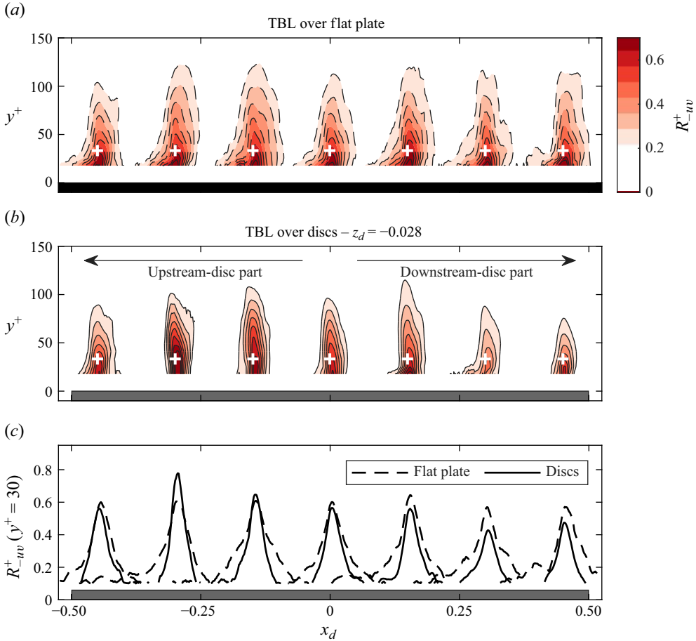
Figure 13. Spatial distribution of the two-point covariance R_{-uv}^+ , defined in (4.3). White plus markers indicate reference locations x_{d,ref} = [-0.45 : 0.15 : 0.45] and y_{ref}^+ = 30 . (a) Contour for the flat-plate case. (b) Contour for the rotating-disc case at z_d = -0.028 . (c) Streamwise profiles at y^+ = 30 for the flat-plate (dashed line) and rotating-disc (solid line) cases. Black and grey rectangles denote the flat-plate and the disc surfaces.
