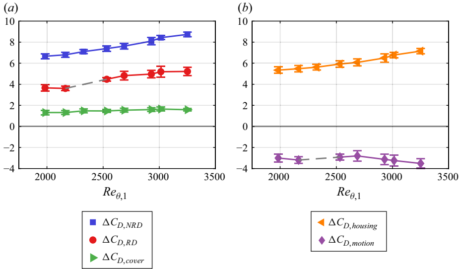
Figure 5. Percentage difference in drag coefficients with respect to the reference flat-plate case as a function of Re_{\theta,1} . Error bars denote the 95 % confidence interval (refer to § 2.3).
