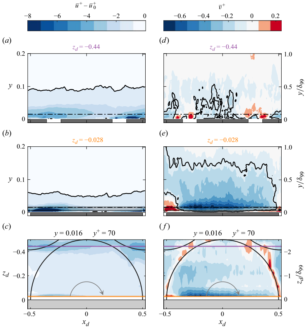
Figure 9. Contours of the disc-induced mean-flow (a–c) streamwise-velocity deficit and (d–f) wall-normal velocity. x_d - y contours at (a, d) z_d = -0.44 ( z_d^* = -40 mm), (b, e) z_d = -0.028 ( z_d^* = -2.5 mm) and (c, f) x_d - z_d contours at y = 0.016 ( y^* = 1.5 mm). The wall-normal height of (c, f) is indicated by the dash-dotted lines (a, b, d, e). The coloured lines in (c, f) denote the spanwise location of (a, b, d, e) and match the title colour accordingly. The dark grey regions in (a, b, d, e) represent the cross-section of the rotating discs. The transparent grey regions in (b, e) represent the cross-section of the covering plates. The light grey region in (c, f) indicates the cover. The black contour lines in (a–d) indicate the y location at which the flow modification penetrates and correspond to 5% of the minimum value within the measurement volume, i.e. 0.05 \cdot \min[\bar{u}^+(x, y, z) - \bar{u}_0^+(x, y, z)] and 0.05 \cdot \min \bar{v}^+(x, y, z) .
