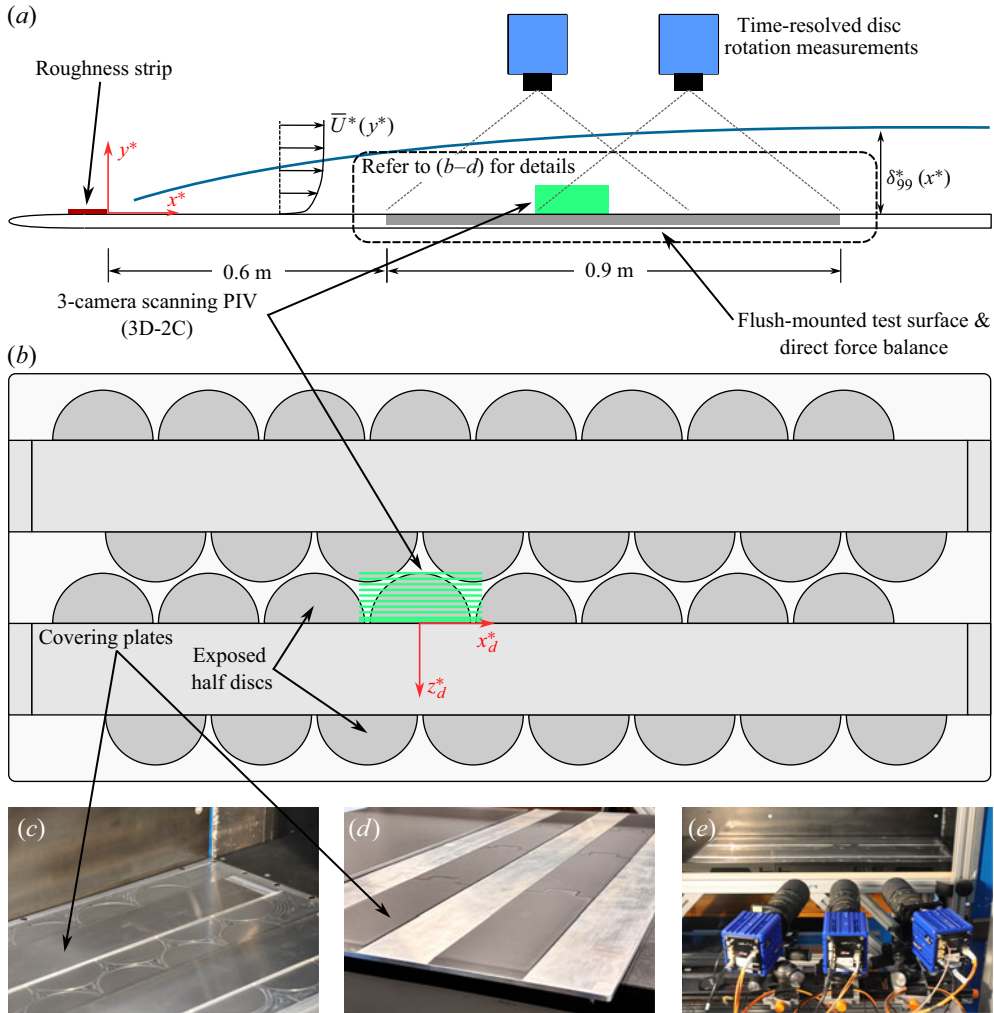
Figure 1. (a) Side-view schematic of the experimental set-up. (b) Top-view schematic of the rotating-disc surface and the 10 scanning-PIV planes arranged along the span (PIV stands for particle image velocimetry). The photographs show (c) the rotating-disc surface near the leading edge of the model, (d) the test surface featuring the covering plates only and (e) the three-camera PIV set-up. A movie of the rotating discs is available in the supplementary material is available at https://doi.org/10.1017/jfm.2026.11917 . Here 3D-2C is three-dimensional two-component.
