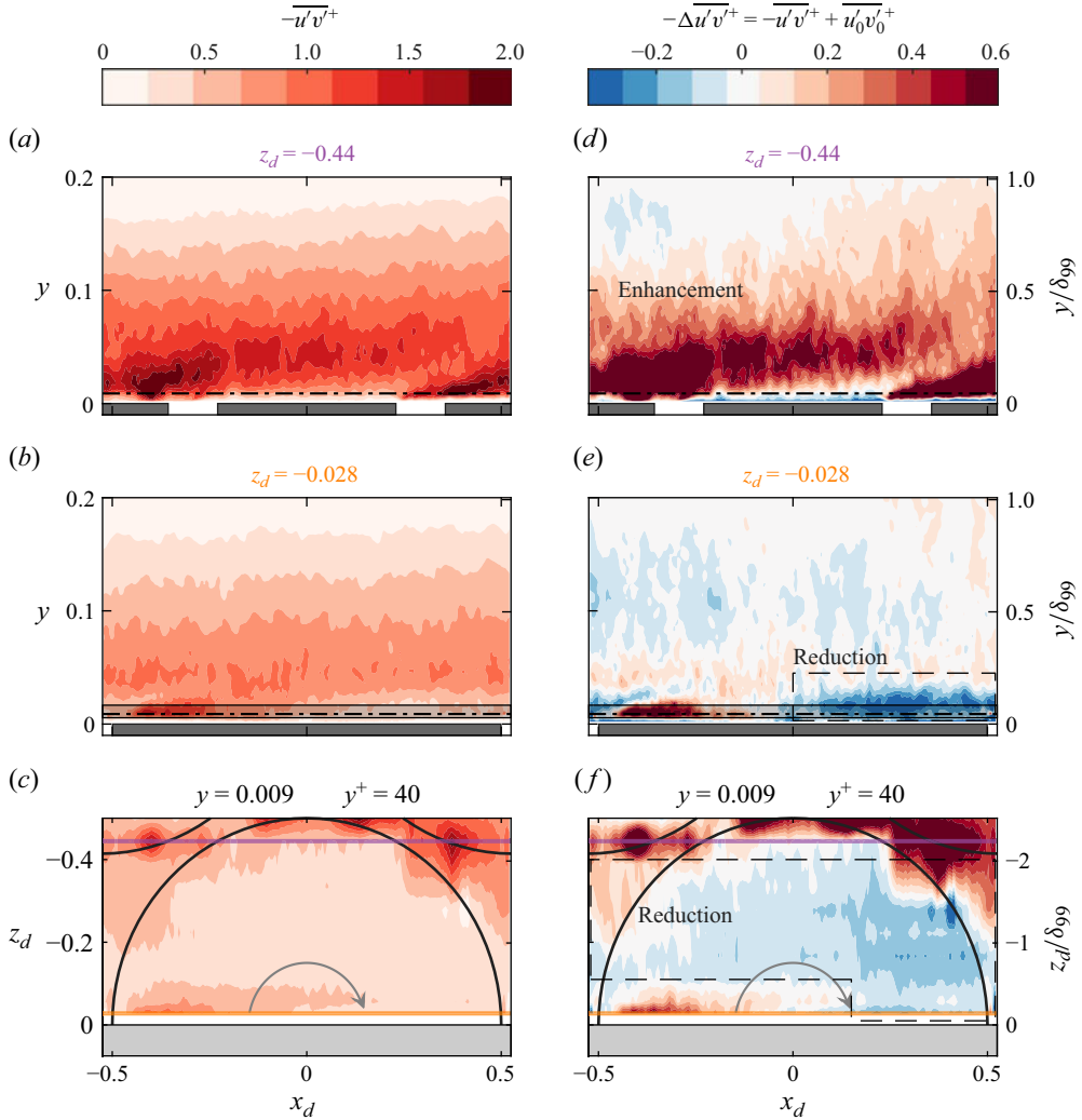
Figure 14. Contours of the (a, b, c) Reynolds stresses, -\overline{u'v'}^+ and (d, e, f) their difference to the flat-plate reference, -\Delta\overline{u'v'}^+ . The flat-plate component is streamwise averaged to reduce the impact of statistical noise. The layout is the same as that of figure 9.
