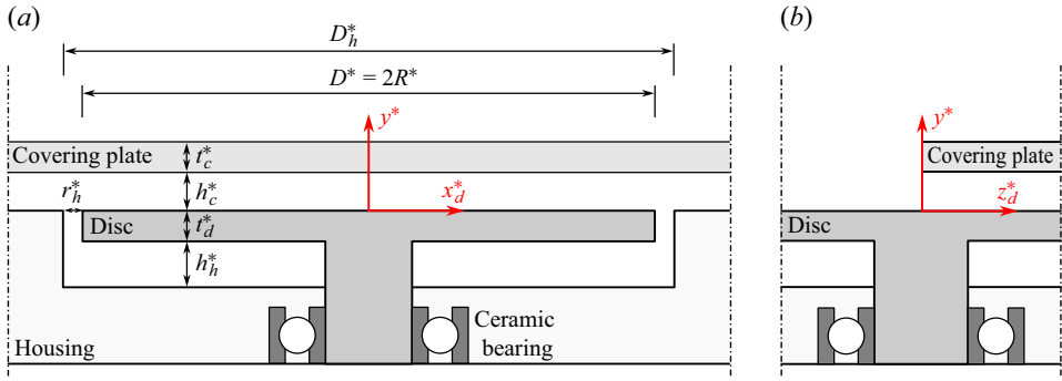
Figure 2. Schematic diagrams of a disc and its housing. The relevant dimensions are given in table 1. The distances are not to scale. (a) Side view in the x_d^* - y^* plane and (b) cross-section view in the y^* - z_d^* plane.
