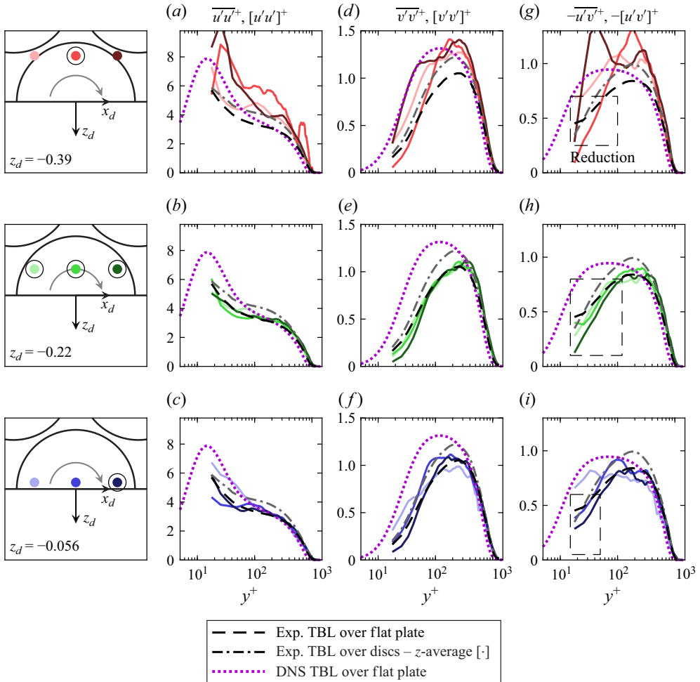
Figure 11. Wall-normal profiles of turbulent stresses, viscous scaled with u_{\tau,d}^* of the flat plate, of (a–c) streamwise normal stresses, (d–f) turbulent wall-normal normal stresses and (g–i) Reynolds shear stresses. The dashed boxes in (g–i) show the near-wall region where the Reynolds shear stresses are reduced. Their (x_d, z_d) locations are marked by the circles in the schematics in the left column. The layout and the line styles correspond to figure 8.
