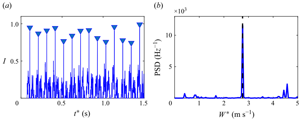
Figure 3. (a) Time series of the indicator ( I ) for the measurement of the disc angular velocity. The triangles denote the result of the peak detection algorithm. (b) Power spectral density of the indicator and time-averaged disc tip velocity, denoted by the vertical dashed line.
