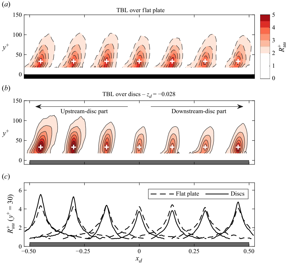
Figure 12. Spatial distribution of the two-point variance R_{uu}^+ , defined in (4.2). White plus markers indicate reference locations x_{d,ref} = [-0.45 : 0.15 : 0.45] and y_{ref}^+ = 30 . (a) Contour for the flat-plate case. (b) Contour for the rotating-disc case at z_d = -0.028 . (c) Streamwise profiles at y^+ = 30 for the flat-plate (dashed line) and rotating-disc (solid line) cases. Black and grey rectangles denote the flat-plate and the disc surfaces.
