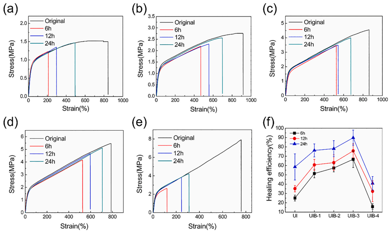
Fig. 6. Strain-stress curves of original and healed self-healing materials after different healing times at room temperature ((a)–(e): UI, UIB-1, UIB-2, UIB-3, UIB-4), the corresponding healing efficiency of the self-healing materials tested (f).
