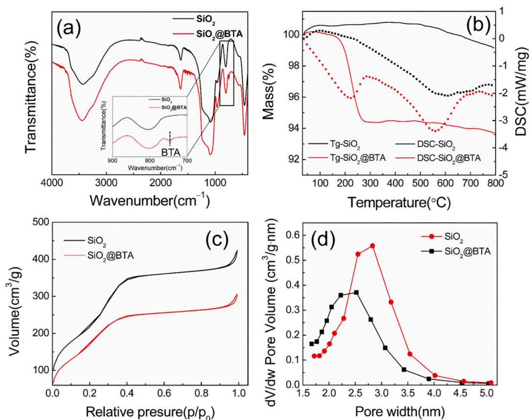
Fig. 2. Characterization of \text{SiO}_2 and \text{SiO}_2\text{@BTA} : (a) FTIR spectrum. (b) TG and DSC curves. (c) \text{N}_2 sorption isotherm. (d) Pore size distribution.
