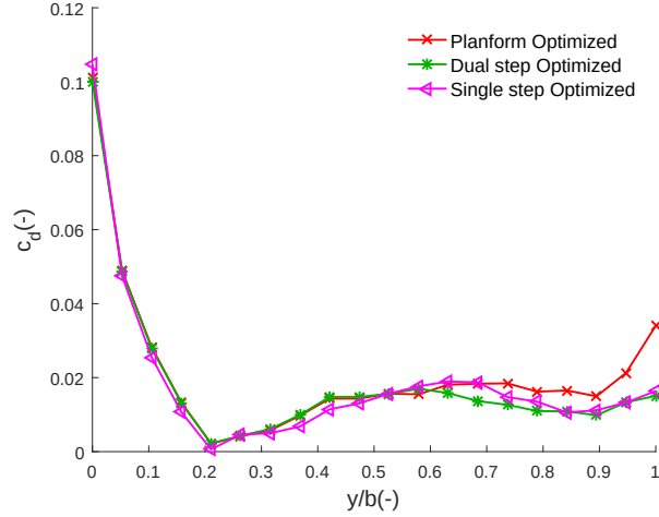
Figure 17. Local inviscid drag coefficient distribution: comparison between airfoils-optimized configuration and planform-optimized one
