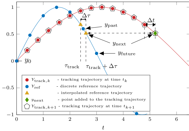
Fig. 9. Warping NMPC shifting strategy for \mathbf{y} = [y] \in \mathbb{R}^1 : \tau_{\text{track}} is used to follow the last point of \mathbf{Y}_{\text{track}} within the reference trajectory \mathbf{y}_{\text{ref}} .
