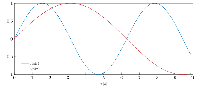
Fig. A.15. Warping of a sin trajectory with \dot{w}(t) = \frac{1}{2} .
