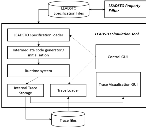
Fig. 8: LEADSTO architecture [45]
