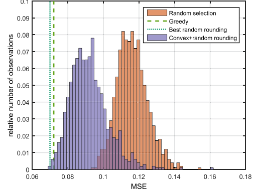
Fig. 9. MSE distribution for the problem of Section IV-B, for a set of 1000 randomly generated masks, as well as 1000 masks generated using the proposed random rounding procedure, and the MSEs of the proposed methods.
