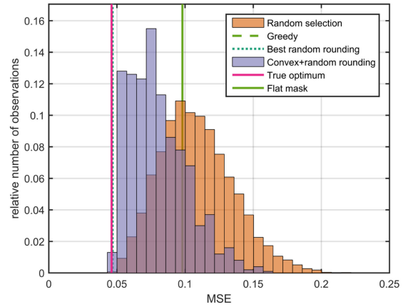
Fig. 6. MSE distribution for the problem described in Section IV-A. We show the MSE distribution for a set of 10,000 randomly generated masks, and 10,000 masks generated using the proposed random rounding procedure, the MSEs of the proposed methods, the MSE of the best mask, as well as a flat mask.
