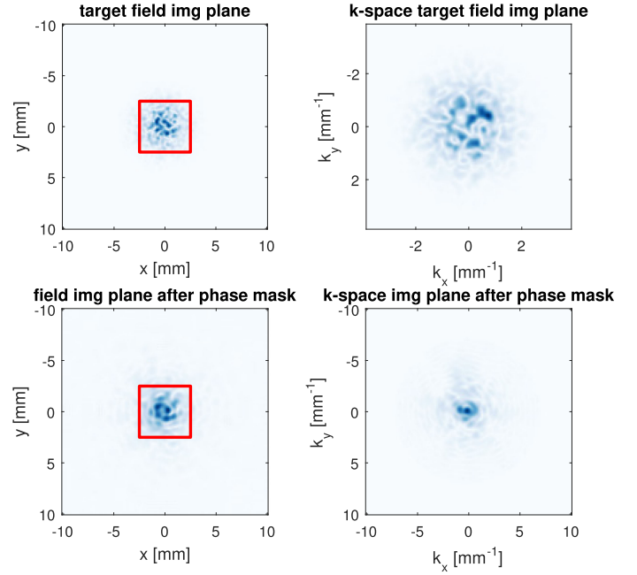
Fig. 22. Top: Target pressure field for f = 4 MHz in the image plane. Bottom: The field in the image plane produced with the mask obtained through the IASA method. All figures show the magnitude of the complex pressure fields. The red box indicates the pixel ROI used for optimization in Section IV-C.
