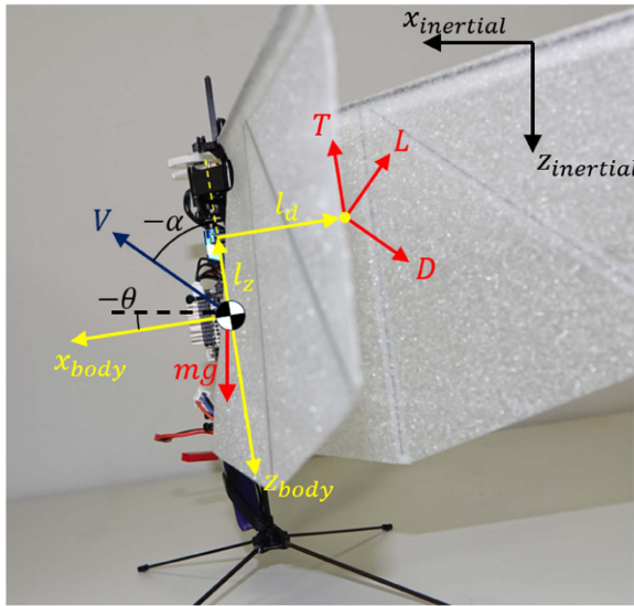
Fig. 2. Scheme of variables and forces over the FWMAV.
