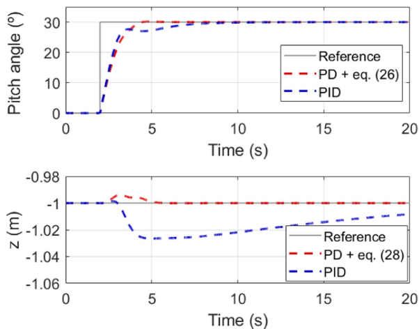
Fig. 7. Transient of the pitch angle and the height for a reference of 30^\circ .
