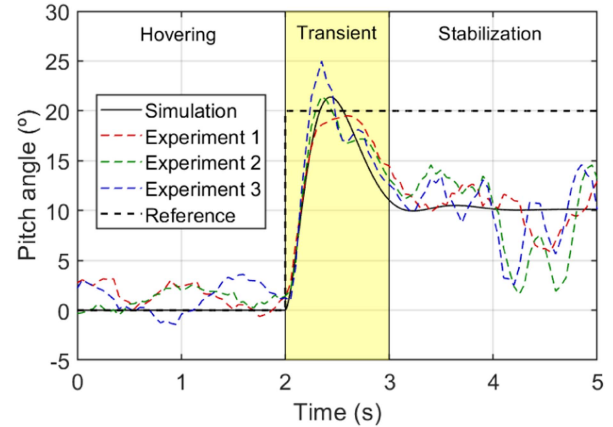
Fig. 5. Evolution of the pitch angle for a step pitch control signal of 20^\circ .
