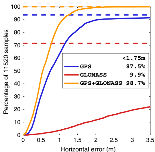
Fig. 9 Cumulative distribution of horizontal position errors for kinematic processing of stationary experiment with a 30^\circ elevation mask angle. The GPS + GLONASS error is 98.7% of the time still smaller than 1.75 m; GPS 87.5%, GLONASS-only 9.9%. About 6.3% of the time a GPS solution is not available at all; 28.5% of the time for GLONASS
