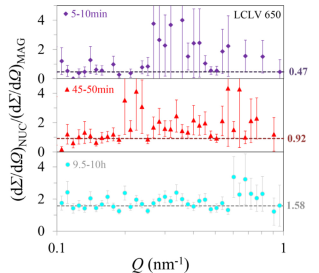
Fig. 3. Ratios of the nuclear to magnetic scattering cross sections plotted versus the scattering vector, Q , on a logarithmic scale, for LCLV alloy samples annealed at 650 °C for different annealing times from the in-situ scattering curves of Figs. 2a and b.
