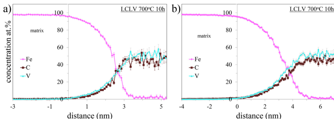
Fig. 11. Representative proximity diagrams of two precipitates differing in stoichiometry in the LCLV steel annealed at 700°C for 10 h. In a), the carbon-to-metal ratio is closer to the stoichiometric ratio than in b).
