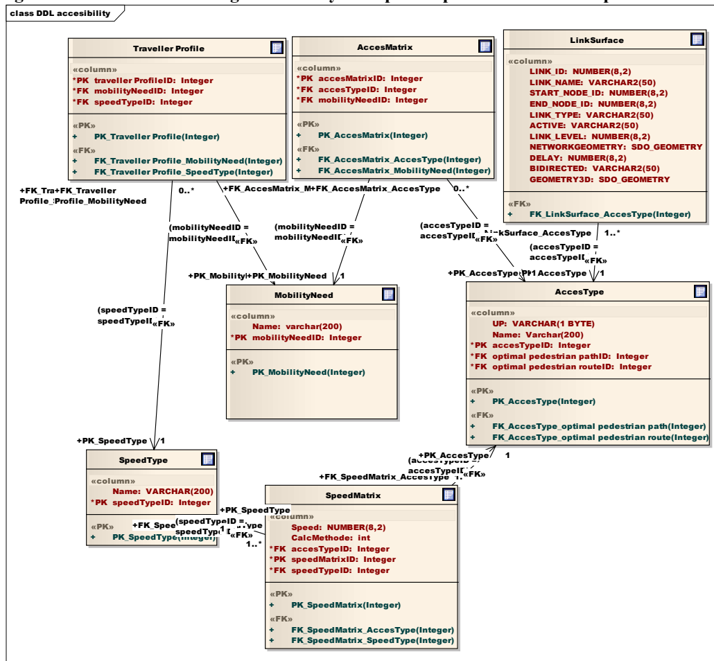
Figure 36 DDL to create tables relating accessibility and speed aspects from traveller profile to LinkSurface.
