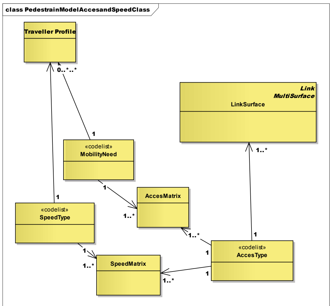
Figure 29 Class diagram accessibility and speed are modelled similar
