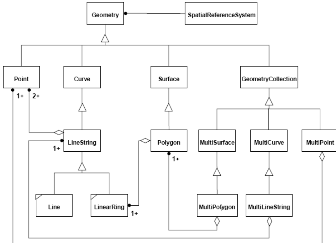
Figure 5 Point, line (String) and Polygon as basis for the simple Feature Specifications for SQL (OGC 1999)
