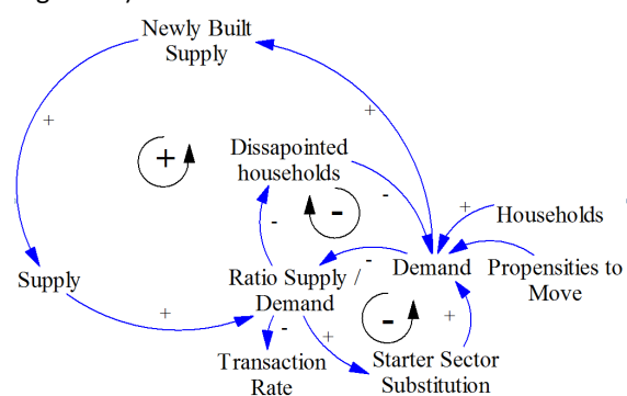
FIGURE 1: GENERAL STRUCTURE OF THE MODEL
