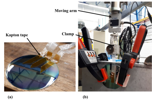
Figure 3. Sample (a) before and (b) after installation in the peel test machine.
