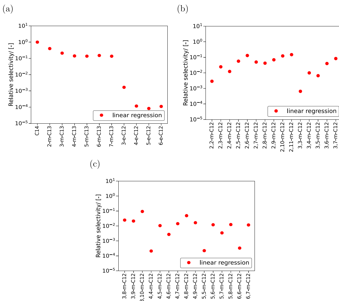
Figure 5. Selectivities of different C_{14} isomers relative to n\text{-}C_{14} at reaction equilibrium in MTW-type zeolite at infinite dilution and 500 K. The LR model is used to predict (G_0 - H_0) (0 K) at 500 K and \Delta_f H_0 at 0 K which are used to compute the ideal gas chemical potentials of C_{14} isomers. These chemical potentials are used to compute the gas phase reaction equilibrium distribution of hydroisomerization of C_{14} . The raw data is listed in the Excel worksheet xi_iC14_500 K of the Supporting Information SI4.xlsx.
