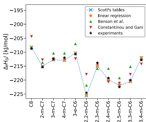
Figure 3. Prediction of \Delta_f H_0 for C_8 isomers at 298.15 K using the LR model, Benson et al.'s group additivity method, 18 Constantinou and Gani's group contribution, 20 the Scott's tables, 9 and the experimental data listed by Scott. 10 The predictions using the LR model are in excellent agreement with the Scott's tables and the data from the experiments. 10 For the \Delta_f H_0 values of C_8 isomers at 298.15 K, using the experimental data as the reference, the Mean Absolute Errors (MAEs) are the smallest for our LR model (0.62 kJ/mol) and the Scott's Tables (0.64 kJ/mol). This is followed by Constantinou and Gani's group contribution method (2.04 kJ/mol), and Benson et al.'s group additivity method (2.37 kJ/mol) respectively. The dashed blue line through the data points obtained from the Scott's tables is a guide to the eye.
