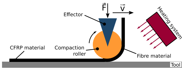
Fig. 1 AFP manufacturing process using a heating system to apply temperature and a compaction roller to apply pressure to the laid up fibre material. \mathbf{F} is the compaction force and \mathbf{v} the effector velocity
