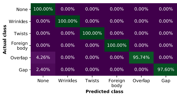
(e) DS training: AUG_GT_All; DS test: RE_All from Table 8 run 1.3
