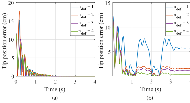
Fig. 2. Tip position estimation error using 1 actuator. (a) The same model dimension was used for both the dynamic model and the algorithm implementation. (b) We implement our algorithm in a high model dimension model.
