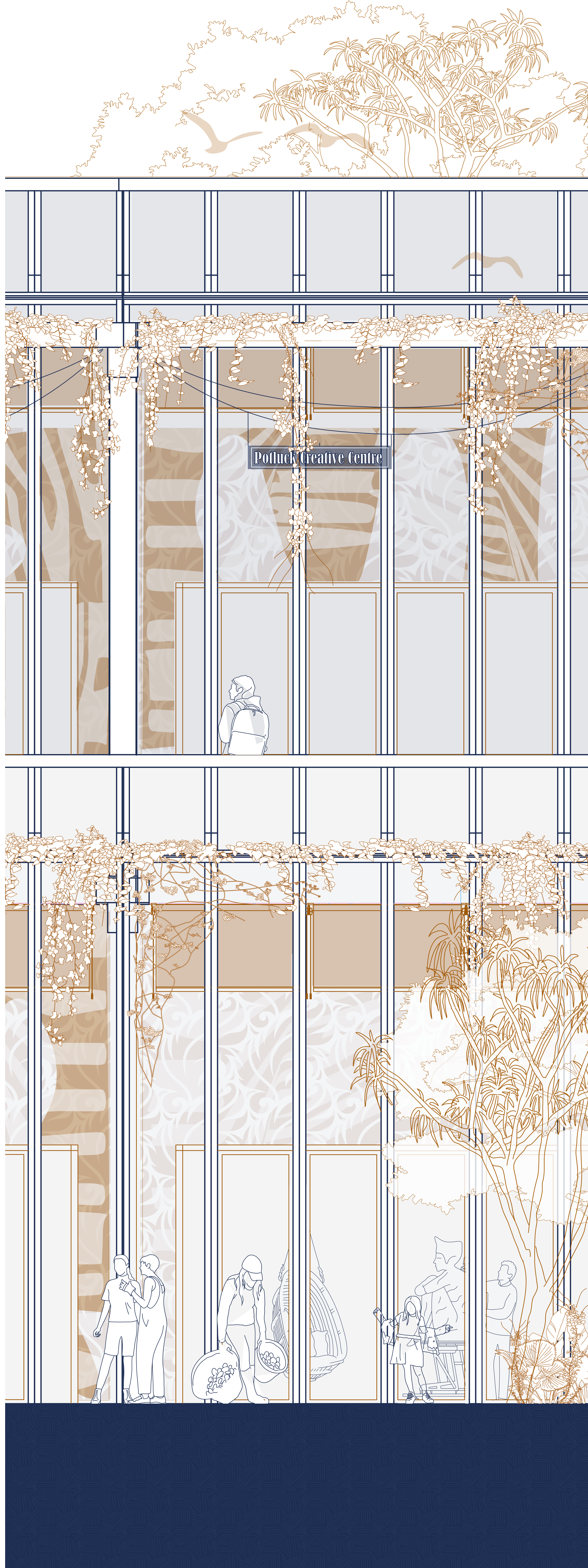
1:20 Combination Drawing of Workshop Area Elevation, Cross Section and Plan Section
