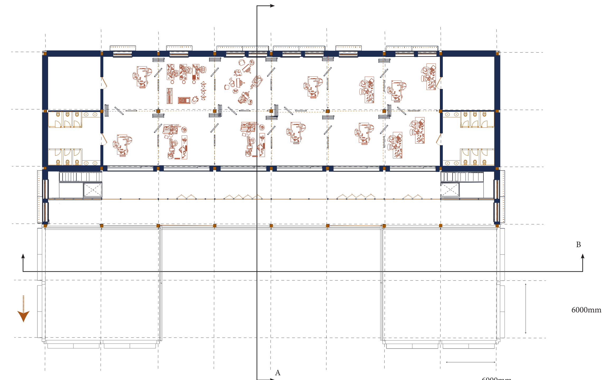
First Floor Plan 1:200
