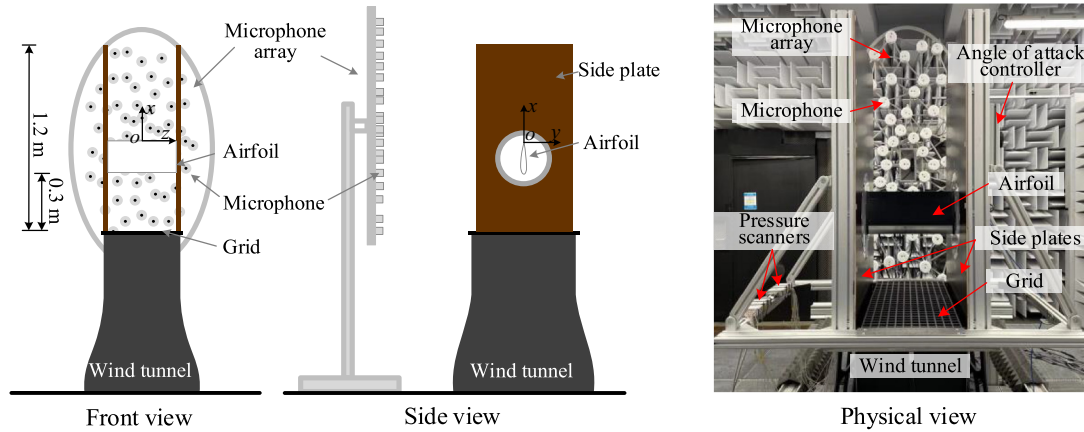
Fig. 1. Experimental setup.
