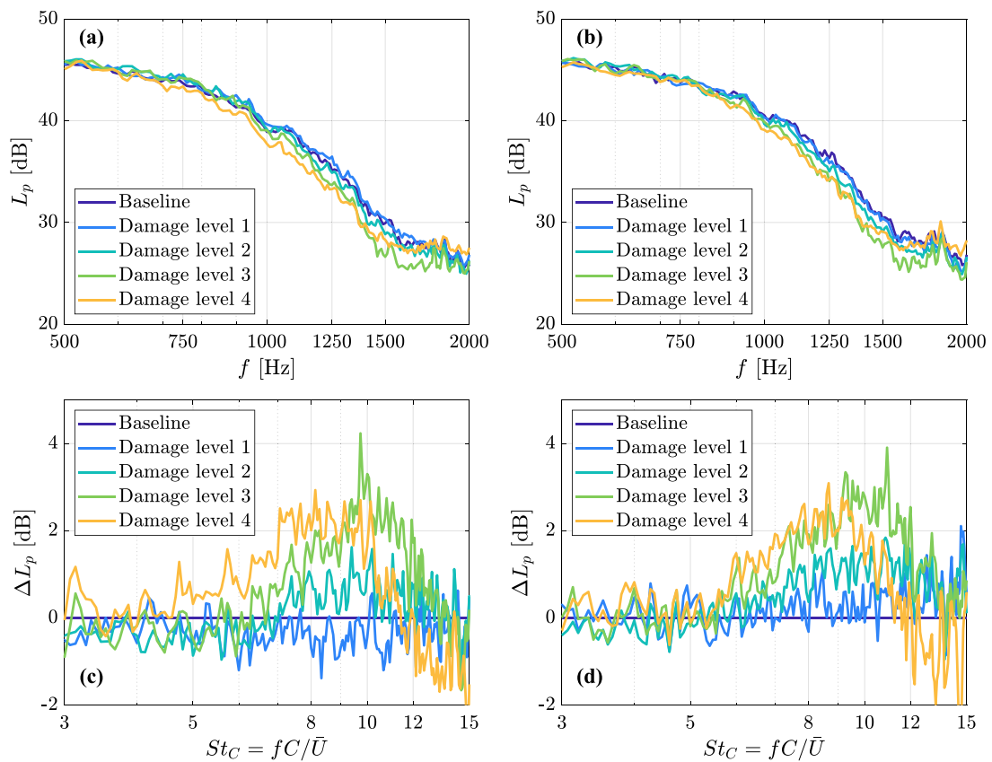
Fig. 11. Spectra of sound pressure level and spectral differences compared to the baseline at the leading edge for different damage levels at an angle of attack of 0^\circ when grid #1 is mounted with a mean flow velocity of 30 m/s: (a), (c) on the suction side and (b), (d) on the pressure side.
