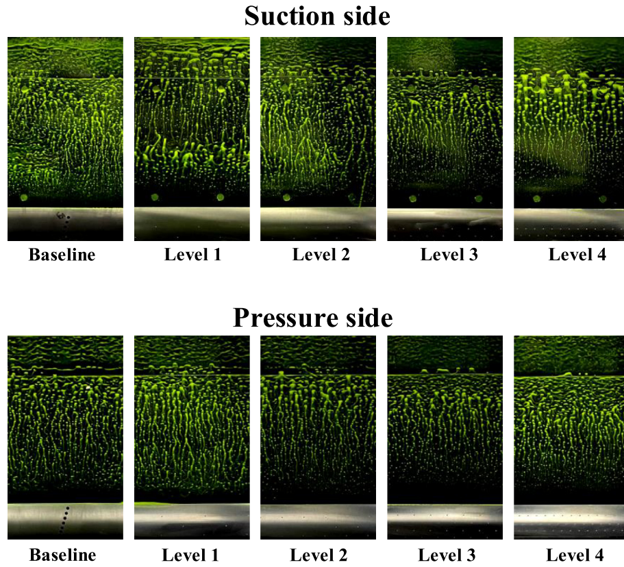
Fig. 10. Surface oil flow visualization for different damage levels at an angle of attack of 0^\circ when grid #1 is mounted with a mean flow velocity of 30 m/s.
