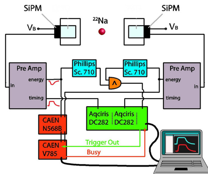
Fig. 7. Schematic representation of the coincidence setup.
