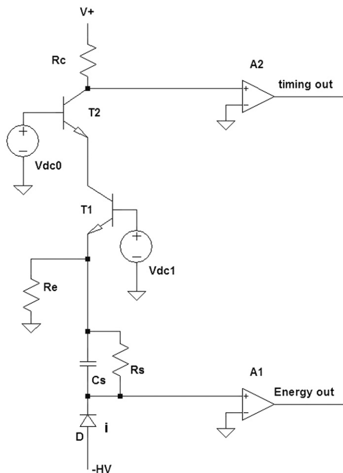
Fig. 6. Simplified circuit of the common-base SiPM amplifier built and tested in this work.
