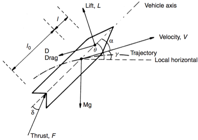
Figure 1.4: Configuration and nomenclature for rocket motion in the vertical plane (Fortescue et al. (2011))
