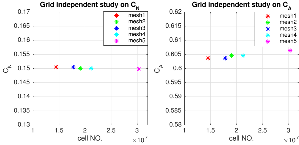
Figure 4.2: Grid independence study of axial, normal force and pitching moment coefficient, @Ma 1.189
