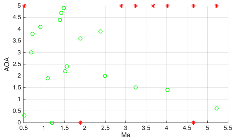
Figure 5.18: Initial LHS and extra added points during the C_A Co-Kringing process; green circle and red asterisk representing LHS sample and extra-added point, respectively
