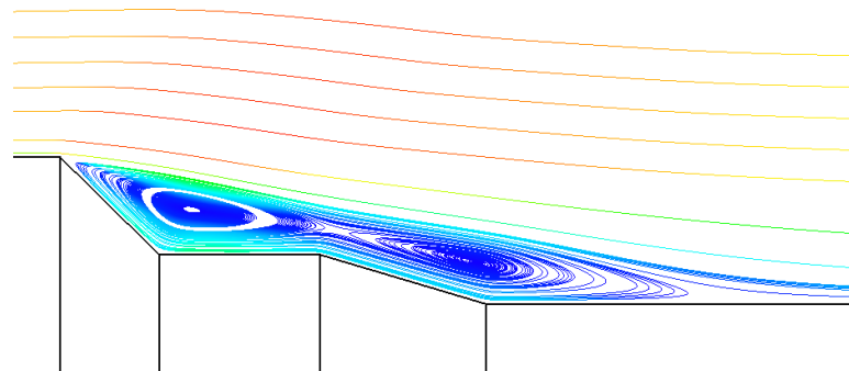
Figure 4.9: Recirculation near the double backward facing steps of Taurus, @Ma 2.41 and AoA 2 Deg
