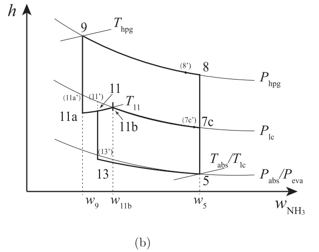
Fig. 5. The state points (referring to the points shown in Fig. 4) of the solution stream plotted in a \ln P - (-1/T) diagram (a) and an h - w diagram (b). Points 11, 11a and 13 sharing the same pressure and fraction with points 11', 11a', and 13', respectively, are at subcooled conditions. Points 7c and 8 have a possibility of refrigerant boil off, the portions of saturated solutions are denoted as 7c' and 8', respectively.
