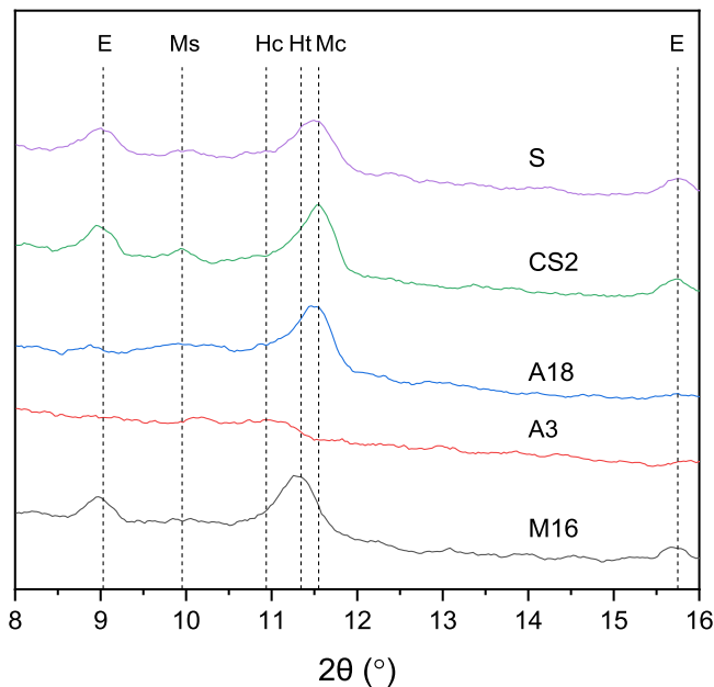
Fig. 8. XRD diffractograms of the selected model pastes after 7 days curing at 40 °C. E – ettringite; Ht: hydrotalcite-like phase; Hc: hemicarbonate; Mc: monocarbonate; Ms: monosulfate.
