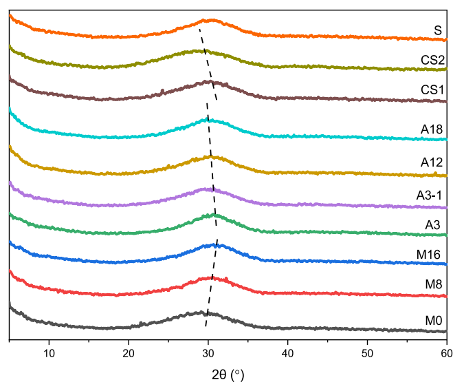
Fig. 2. XRD scans of nine synthetic slags and one commercial slag. The small Bragg peaks in slag M8 and CS1 could be attributed to the formation of akermanite and gehlenite, respectively.
