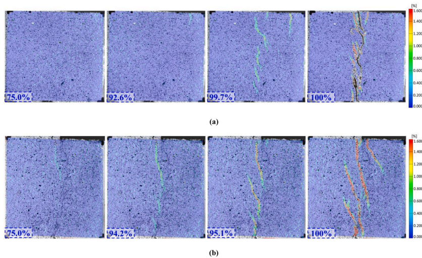
Fig. 14. Typical development process of crack pattern in the interfacial direct shear tests (a) Specimen with chiseled interface (VNIIIIE) (b) Specimen with grooved interface (VNIVE) (Percentage marked in the figures is the ratio of the corresponding load at each cracking state to the ultimate load P_u ).
