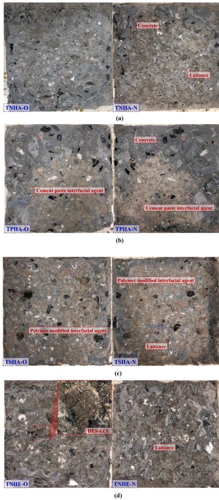
Fig. 10. Section morphology of the interfacial splitting specimens after tests (a) TNIIA (b) TPIIA (c) TSIIA (d) TNIIIE ("O" represents the existing concrete side, "N" represents the HES-ECC side).
