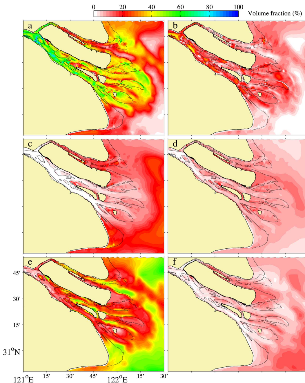
Fig. 6. Spatial distributions of the initial sediment volume fraction in the 2002–2010 hindcast case achieved using the Bed Composition Generation approach (Van der Wegen et al., 2011b): (a) s1 fraction, (b) s2 fraction, (c) m1 fraction, (d) m2 fraction, (e) m3 fraction and (f) m4 fraction. The 5 m isobaths of 2002 are shown by thin black lines.
