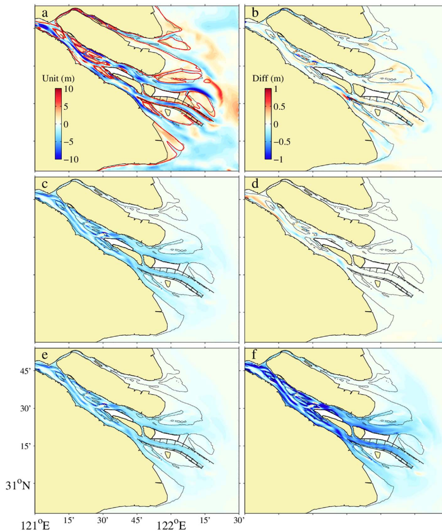
Fig. 13. Erosion and deposition patterns of the forecast (2010–2030) Scenario 4 (a) and the morphological change differences between Scenarios 1 and 0 (b), Scenarios 2 and 0 (c), Scenarios 4 and 3 (e) and Scenarios 5 and 3 (f). (c)–(f) share the range of differences with (b). The thin and thick lines represent the 5 m isobaths of 2010 and 2030, respectively.
