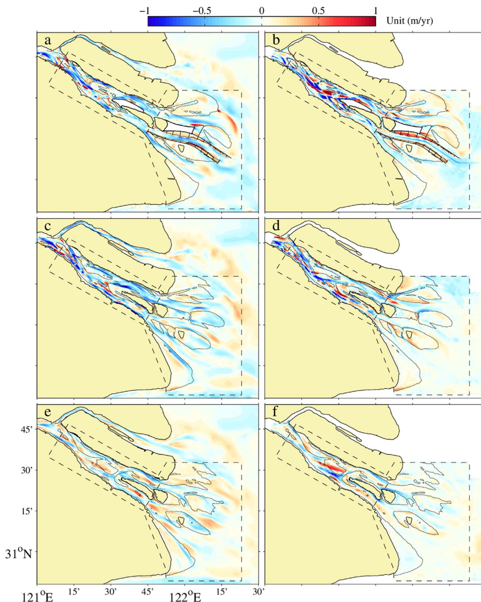
Fig. 10. Modeled (a, c, e) and observed (b, d, f) erosion (negative) and deposition (positive) patterns in the Yangtze Estuary in 2002–2010 (a, b), 1986–1997 (c, d) and 1958–1978 (e, f). The thin solid lines denote the observed 5 m isobaths of the last year, and the dashed lines denote the defined boundaries of the inner estuary and the mouth bar area.
