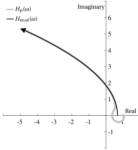
Figure 6.9: Nyquist plot of the apparent dynamics of the active manipulator ( H_p ) and the dynamics of the approximate system ( H_{msd} ).
