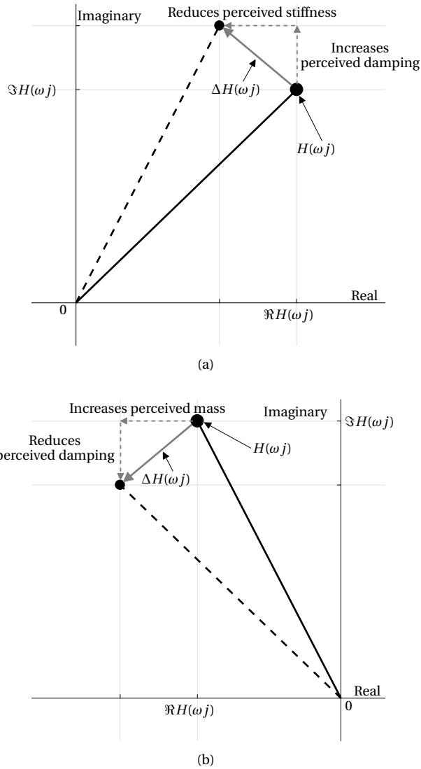
Figure 6.3: An illustration of the changes in the mechanical characteristics perceived by humans, associated with a change in the system dynamics, (a): when \Re H(\omega j) is positive; (b): when \Re H(\omega j) is negative.
