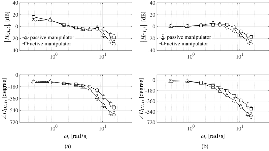
Figure 2.9: Target following frequency responses of subjects (mean \pm std), BW2: (a) open-loop response; (b) closed-loop response
