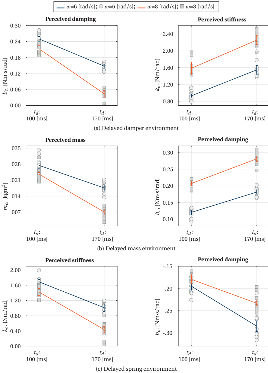
Figure 3.2: Mechanical properties subjects perceived from the delayed reference environments. The data is shown with mean and 95% confidence interval corrected for between-subject variability (represented by the bars). The symbols (square and circle) represent the measurements from individual subjects.
