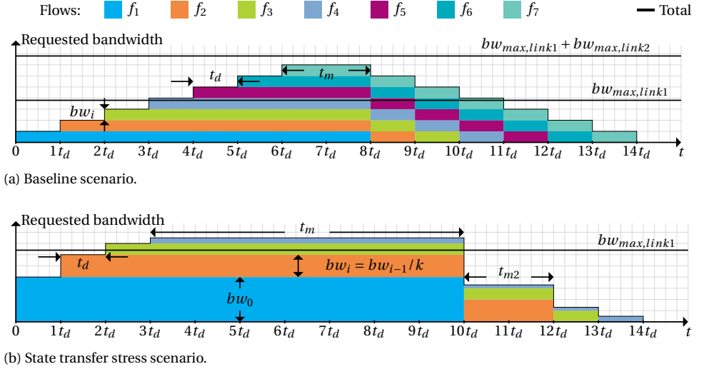
Figure 4.11: Traffic scenarios.
