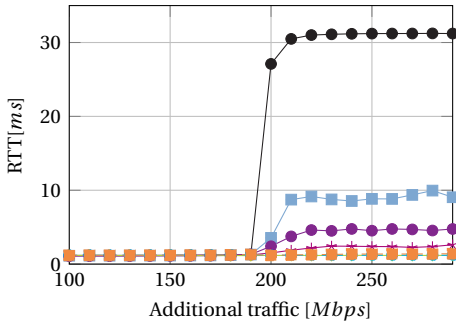
(a) Average RTT for tactile data.
