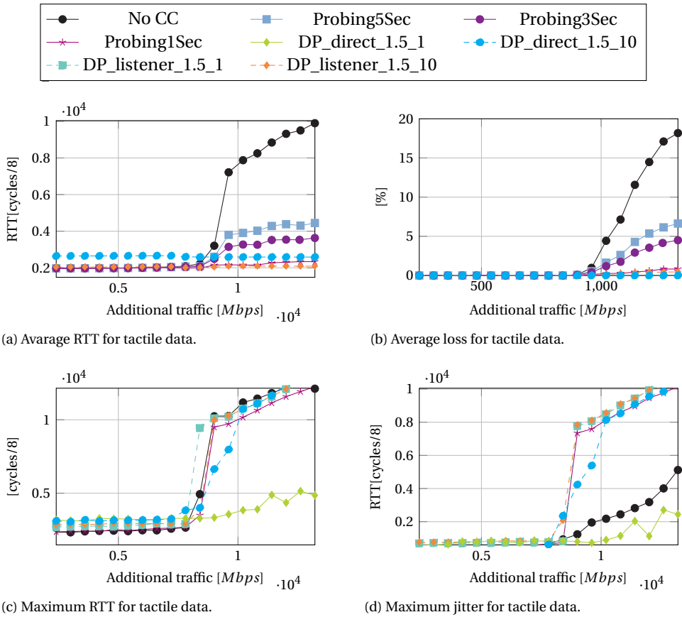
Figure 7.8: Netrnومه SmartNIC scenario (Confidence intervals 90%). Comparison of different QoS parameters for different schemes when additional traffic is generated to create congestion at node s2.
