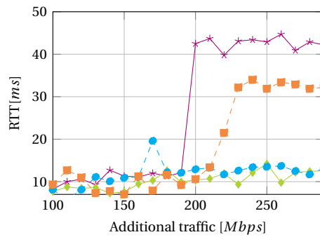
(e) Maximum RTT for tactile data.
