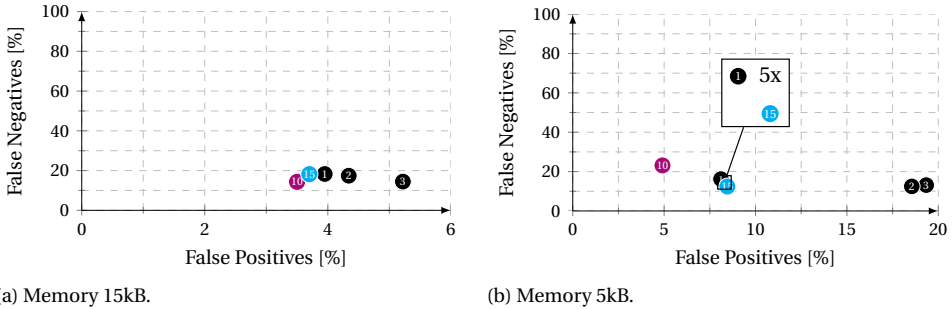
Figure 2.6: Netronome SmartNIC hardware experiments for interval-based schemes using 40 different CAIDA traces.
