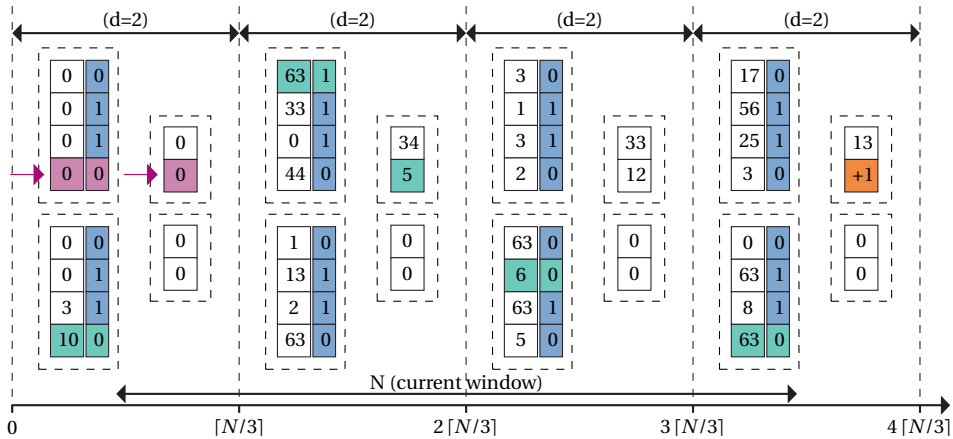
Figure 2.4: Sequential Zeroing scheme, which applies the Zeroing Window technique to the last sub-interval of the Sequential Window. We use the example of Figure 2.2 with k + 1 = 4 sub-intervals, each implementing a Modulo sketch of depth d = 2 . Again, each stage is subdivided into 2 equal-size sub-stages (in dashed rectangles). Assume we want to reset the last (blue) counters of both of the top sub-stages in the left sub-interval that contains the oldest packets. We can indeed do so without violating memory constraints.
