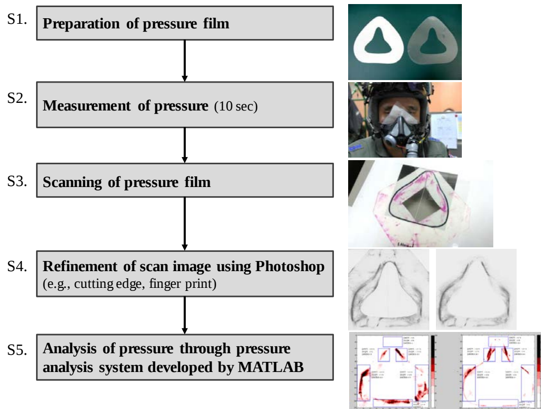
Figure 3. Facial contact pressure measurement and analysis protocol
