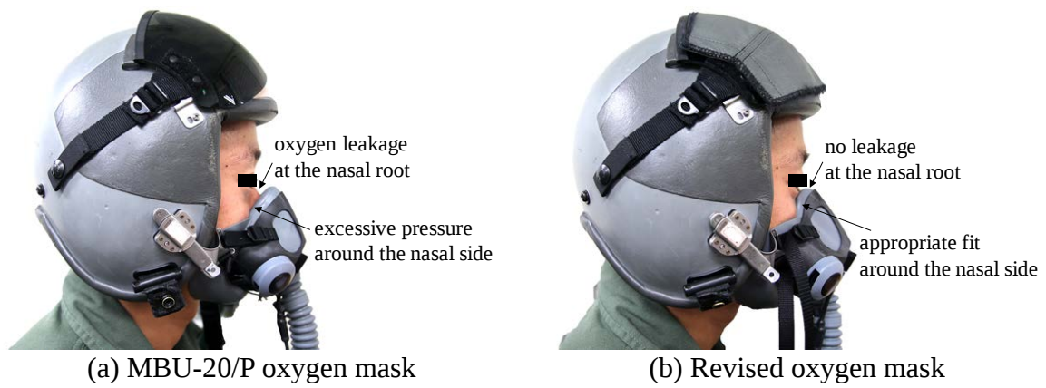
Figure 1. Comparison of existing and revised pilot oxygen masks
