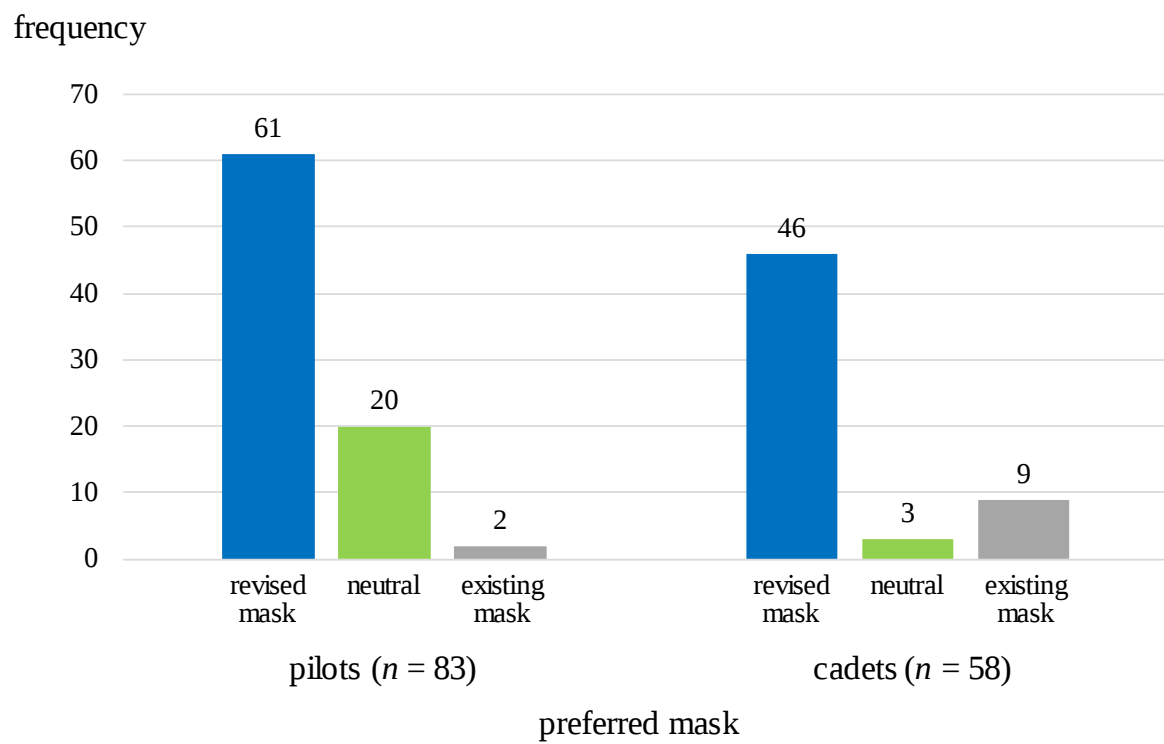
Figure 9. Preference results
