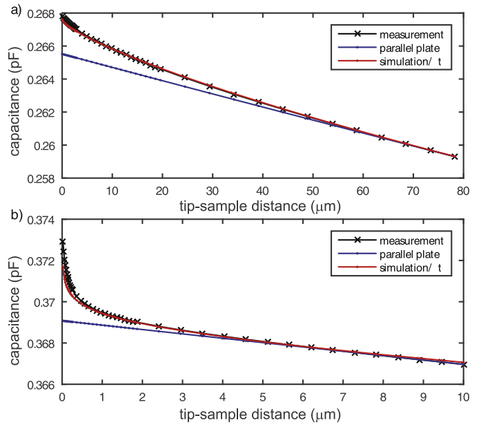
Fig. 8. Comparison between measured, simulated, and analytically calculated data of the tip-sample capacitance. The measurements are shown in black: (a) for the JPE-STM and (b) for the JT-STM. Our simulations (red) closely fit the experimental values. The curve in blue represents an analytical lower boundary based on a parallel-plate approximation.
